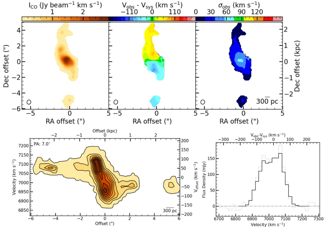
Figure 2. As in Fig. 1, but for HE1108-2813. The spectrum is extracted within a box of 5'' \times 13''.5 .
