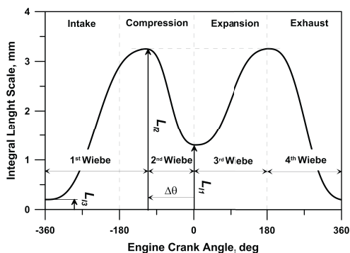
Figure 4. Integral length scale reconstruction.
