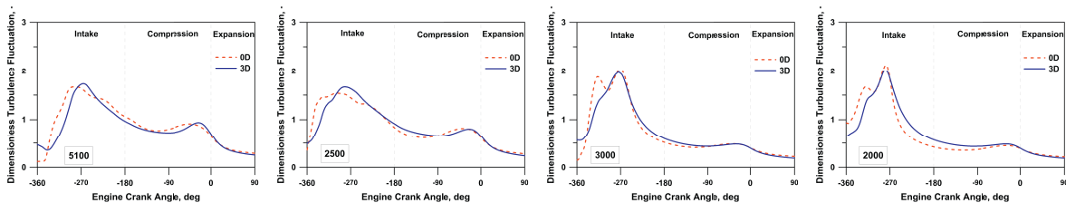
Figure 6. Dimensionless turbulence fluctuation 0D/3D comparison
