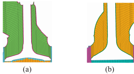
Figure 1. Detail of the intake (a) and exhaust (b) valve curtain grid. 2500FL case
