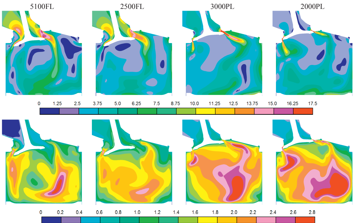
Figure 2. Normalized mean (above) and turbulent (below) velocity @450 CAD
