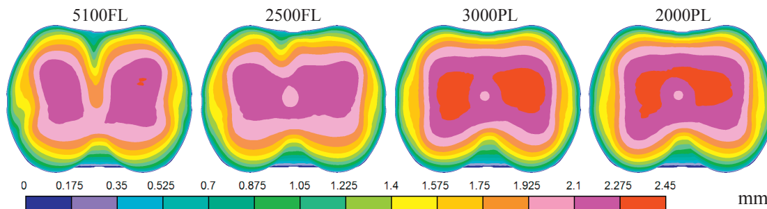
Figure 3. Integral Length scale @720 CAD
