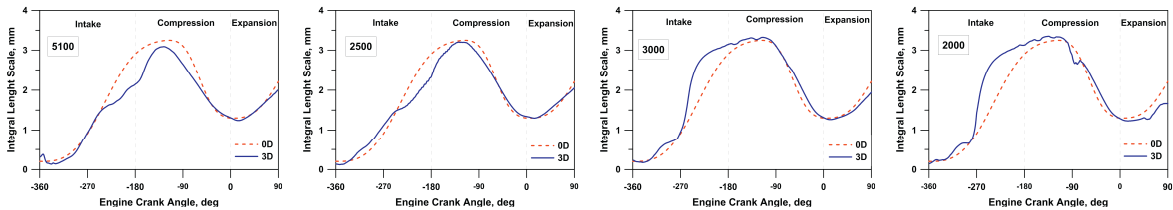
Figure 5. Integral length scale 0D/3D comparison
