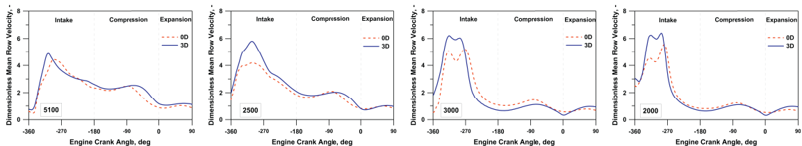
Figure 7. Dimensionless mean flow velocity 0D/3D comparison
