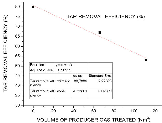
Fig. 5. Tar removal efficiency vs volume of producer gas treated
