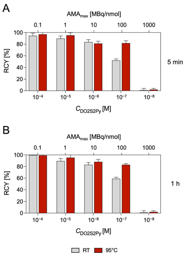
Fig. 10 Concentration- and temperature-dependent ^{111}\text{Ag}[\text{Ag}^+] radiolabeling with DO2S2Py at pH 7.4 after (A) 5 min and (B) 60 min.
