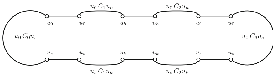
Figure 4. Construction of a Hamilton cycle described in Lemma 3.3. This figure shows the case \lambda = 3 . The paths we consider in each component K_j , 0 \leq j \leq \lambda , are represented by curved lines, the straight line segments represent the edges of type a connecting the vertices in K_j to the vertices in K_{j+1} that are assigned the same label
