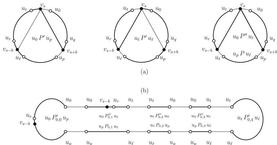
Figure 2. Construction of a Hamilton cycle in G in Case 1 of the proof of Lemma 3.2, when \lambda is even, \mu = 0 , and the connected components of H(m, S) are Hamiltonian. a The bold lines stand for the paths we consider in each component K_j , 0 \leq j \leq \lambda . b We join the paths through edges of type a —represented by the thin lines—as described in the proof of Lemma 3.2. This figure shows the case \lambda = 4 . The same construction can be also used when \lambda is odd and \mu = 0 , by replacing the path u_t P'_{0,\lambda} u_\ell with the path u_0 P'_{0,\lambda} u_p
