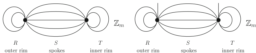
Figure 1. A typical bicirculant B(m; R, S, T) \in \mathcal{B}(m; d, s) , defined by a voltage graph for d - s even (left); for d - s odd a semi-edge is drawn at each vertex (right)
