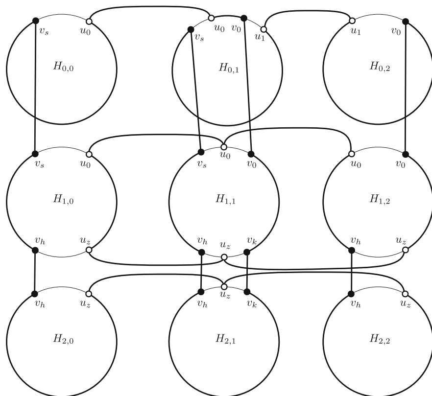
Figure 3. Construction of a Hamilton cycle in G in Case 2 of the proof of Lemma 3.2 when \mu > 0 . In this figure, we have \lambda = \mu = 2
