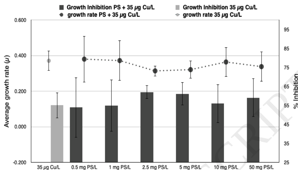
Figure S1: Percentage of growth inhibition compared to control (bars) and average growth rate (circles) of 72 h algal toxicity test of R. subcapitata exposed to Cu (light gray) and Cu (35 µg/L) with increasing PS NPs concentration (dark gray). Data shown as mean \pm standard deviation.
