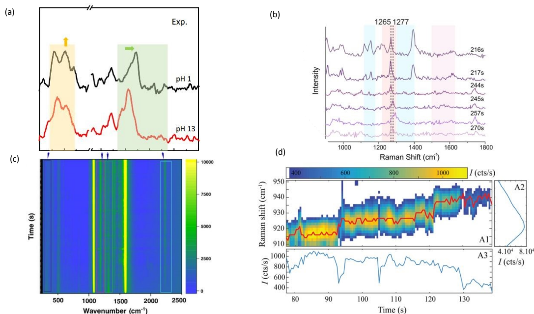
Figure 6 Dynamic interaction or conformation of molecule. (a) SERS spectra of Tyr at pH 1.0 (black) and pH 13.0 (red), respectively. Reproduced with permission from ref (76). Copyright 2023 Springer Nature. (b) SERS spectra showing different time points from a single DONA measurement, highlighting the shift of the Amide III band (blue zones highlight heme unit peaks, the red zone indicates peptide backbone peaks, and the purple zone shows spectral contributions from both). Reproduced with permission from ref (96). Copyright 2024 Springer Nature. (c) Time-series SERS map recorded for 100 s under 633 nm laser excitation showing the transformation of NMSB molecule. Reproduced with permission from ref (82). Copyright 2024 American Chemical Society. (d) Surface enhanced Raman chromatograms of three specific Raman lines of Trp in the single molecule regime. Reproduced with permission from ref (99). Copyright 2019 American Chemical Society.
