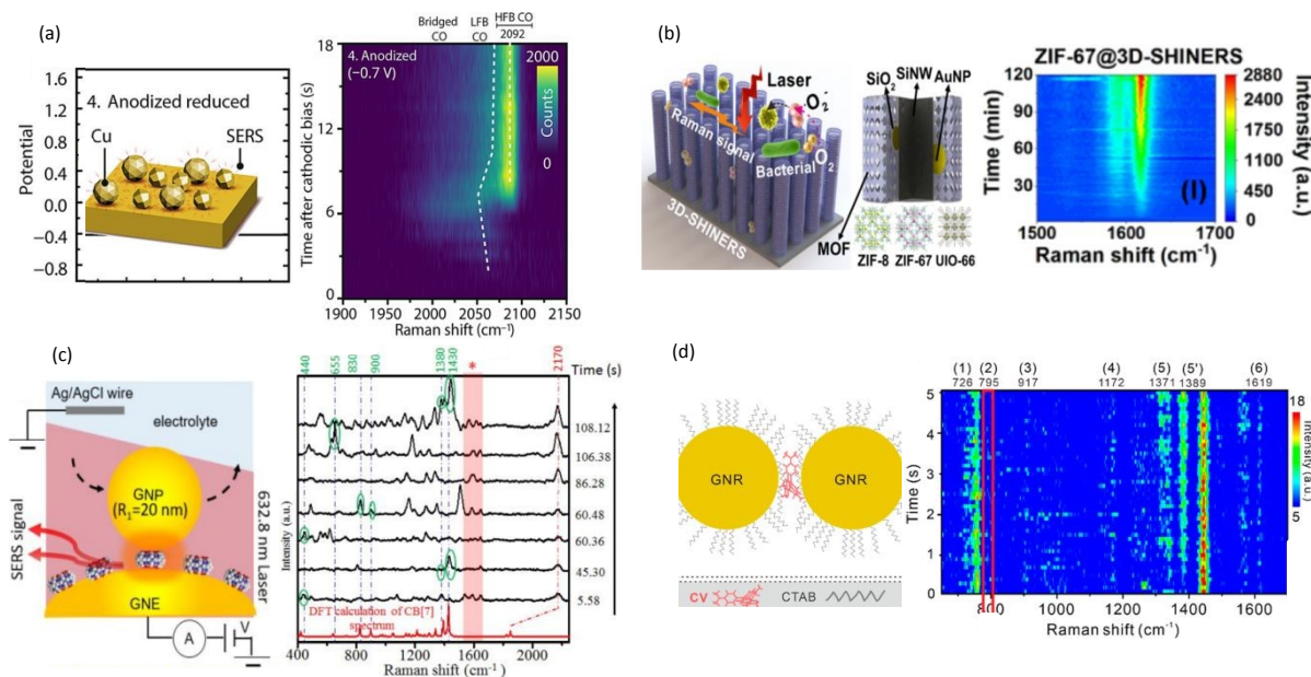
Figure 4 Dynamic SERS researching on (a) Intermediates during chemical reduction, with spectral heatmap from SERS measurements showing the dynamic behaviour of corresponding reduced steps. Reproduced with permission from ref (85). Copyright 2021 Wiley-VCH GmbH. (b) Photocatalysis. Reproduced with permission from ref (31). Copyright 2022 American Chemical Society. (c) Charge transfer between molecular scaffolding to the nanoparticles. Reproduced with permission from ref (87). Copyright 2020 The Royal Society of Chemistry. (d) Single molecular motion at gas/liquid interface. Reproduced with permission from ref (88). Copyright 2023 American Chemical Society.
