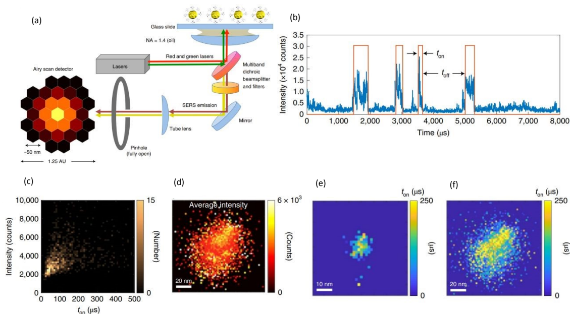
Figure 2 Classical high-speed imaging SERS system and single molecule SIFs. (a) Schematic illustrations of High-speed spectral acquisition system and their experimental approach. Single-molecule SIFs, covered 500\text{ cm}^{-1} to 2000\text{ cm}^{-1} , (b) digitized (d-SIF, shown as a red envelope) to extract time dynamics. (c) Bivariate histogram of the same data showing the SIF intensity versus the d-SIF on time t_{\text{on}} in microseconds. (d) An image of another nanoparticle, this time representing 11,577 individual SIF events, and again showing the occurrence of SIFs all over the single particle. (e) The 32 pixels Airyscan imaging array was used to spatially map the characteristics of the nanoparticle from SM-SERS events. (f) Spatial distribution of t_{\text{on}} for the same particle as in (d). Reproduced with permission from ref (40). Copyright 2019 Springer Nature.
