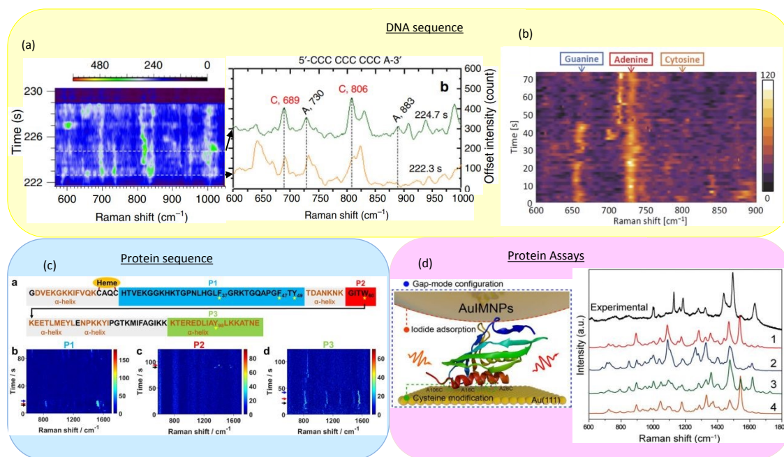
Figure 7 Sequences or structural assays detection with time-dependent SERS spectra. (a) DNA sequence detection by nanopore. Reproduced with permission of ref (55). Copyright 2019 Springer Nature. (b) DNA sequence research from a gold nanoparticle dimer. Reproduced with permission of ref (102). Copyright 2022 Optica Publishing Group. (c) Investigated on protein sequence by a plasmonic structure. Reproduced with permission of ref (56). Copyright 2023 American Chemical Society. (d) Rapidly determining the 3D structure of protein assays. Reproduced with permission of ref (103). Copyright 2023 American Association for the Advancement of Science.
