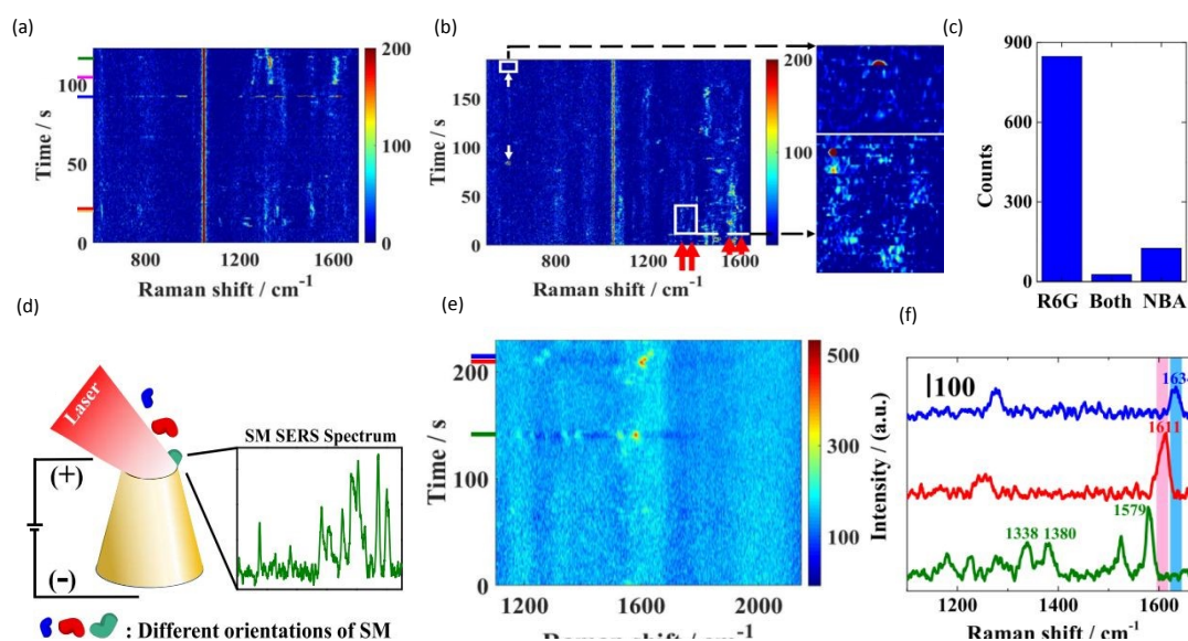
Figure 5 (a-b) Contour graphs of Raman spectra of 10^{-9} M R6G, the mixture of 10^{-9} M R6G and 10^{-9} M NBA under -300 mV with a 0.3 s exposure time respectively; (c) Bi-analyte SERS distribution of R6G and NBA; (d) Conjoint SERS-plasmonic nanopore setup; (e) Contour Raman spectra of 10^{-9} M Hb in a 1 M LiNO 3 (pH 6.6) solution under -300 mV with a 2 s exposure time. The SERS spectra shown in (f) are labeled by short lines with corresponding colors. (f) The SERS spectra extracted from (e) at the time 114, 209, and 211 s, respectively. Reproduced with permission from ref (91). Copyright 2021 American Chemical Society.
