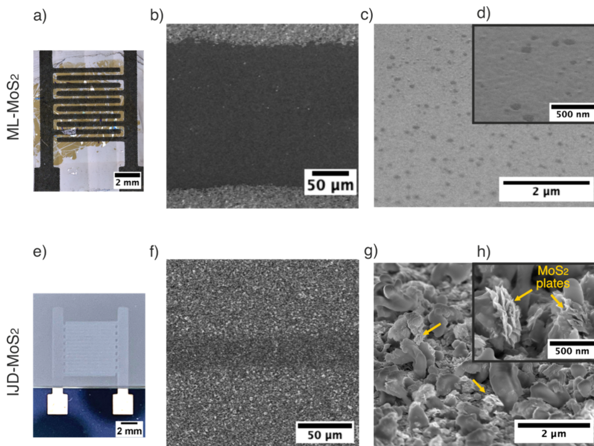
Figure 1. (a) Optical micrograph taken with polarized light of the ML-MoS 2 chemoresistor; (b–d) SEM images in between the IDE spacing of the ML-MoS 2 chemoresistor: (b) top view, (c, d) 54° tilted views with higher magnifications; (e) optical micrograph of the IJD-MoS 2 chemoresistor; (f–h) SEM images in between the IDE spacing of IJD-MoS 2 chemoresistor: (f) top views, (g, h) 54° tilted view with higher magnification showing plate-like MoS 2 structures.
