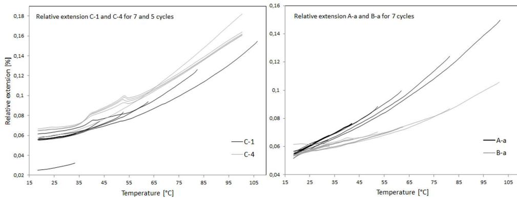
FIGURE 4. Dependence of relative extension on the temperature.
