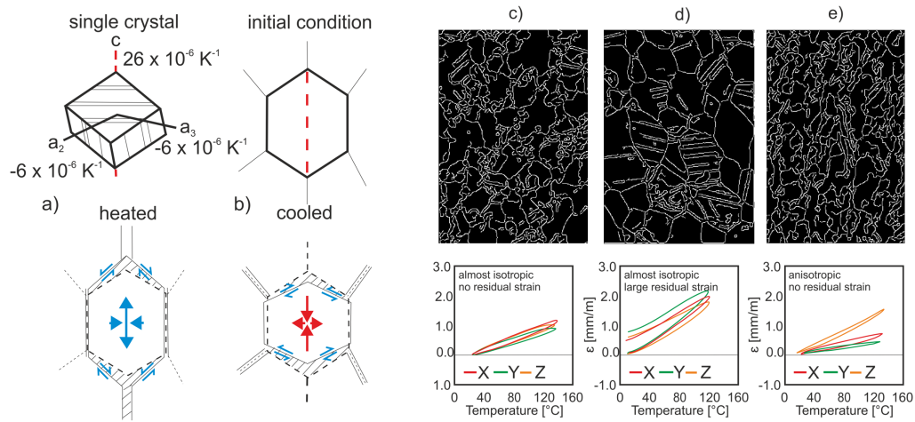
FIGURE 1. Anisotropic thermal expansion of calcite crystals. Adopted from [1].
