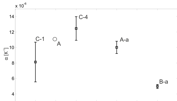
FIGURE 5. Thermal expansion coefficient \alpha of investigated specimens, loaded in the 18-100 °C temperature interval. The value marked "A" represents an average value of \alpha determined by [7] on large set of marble specimens.
