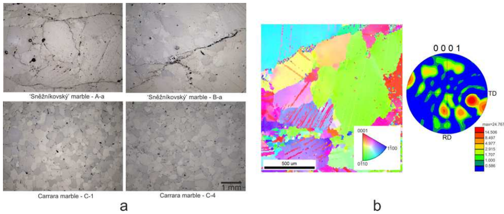
FIGURE 3. a - microfabric of investigated samples, b - orientation of calcite grains in B-a sample.
