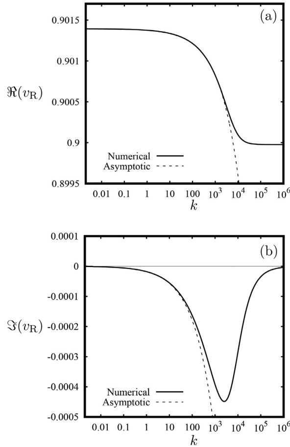
Fig. 1. Dispersion and dissipation of thermoelastic surface waves propagating along the Ox_1 -axis in the Rochelle salt: respectively, real (a) and imaginary part (b) of the phase velocity v_R . The solid curve, representing the numerical solution of the fully coupled thermoelastic system, is superposed onto the asymptotic approximation (33), that appears in dotted style.
