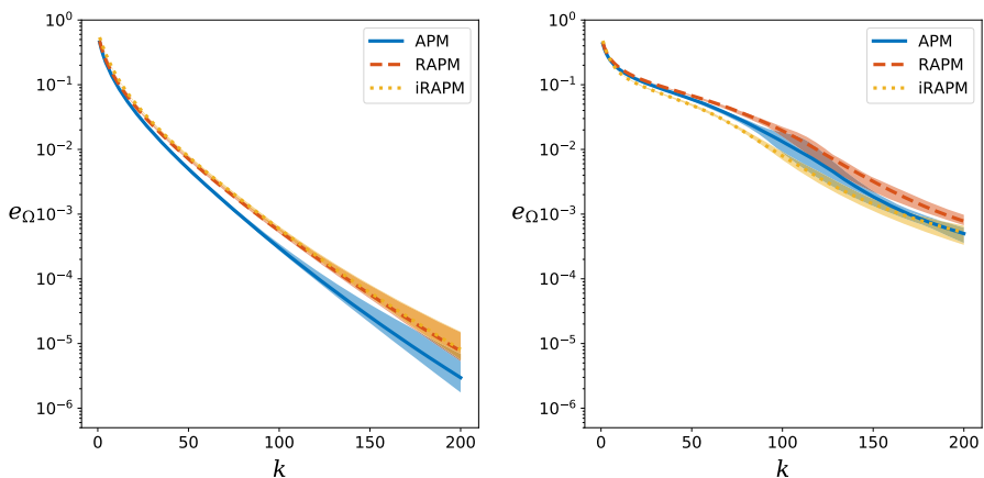
Fig. 3 Mean value and min-max band (over 5 runs) of e_{\Omega} along the iterations. Gaussian matrices (left) and truncated lake (right)
