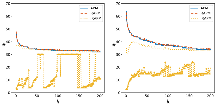
Fig. 5 Number of inner iterations \bar{\ell}_k along outer iterations and number of singular values that satisfy the criterion (4.14). Gaussian matrices (left) and truncated lake (right)
