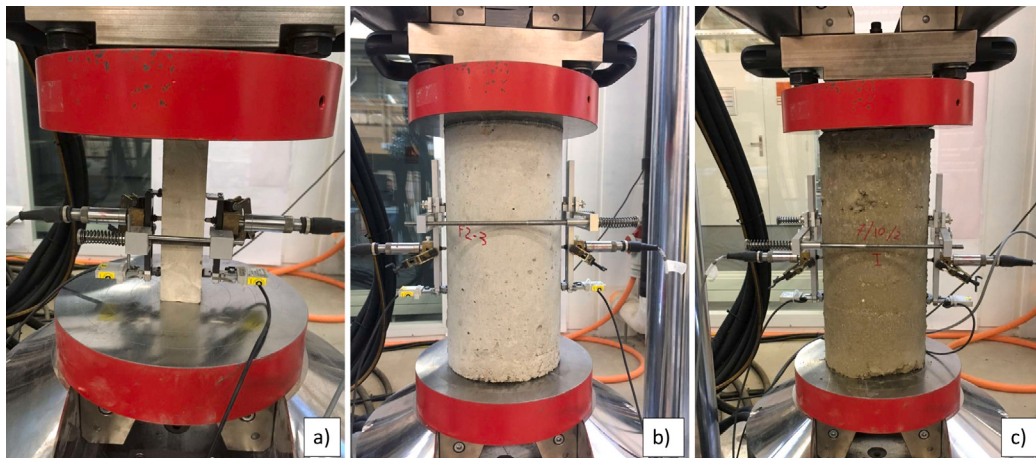
Fig. 7. Experimental test performed on specimens of steps 1(a), 2(b) and 3(c), measuring Young's modulus and Poisson's ratio according to [37,38] respectively.
