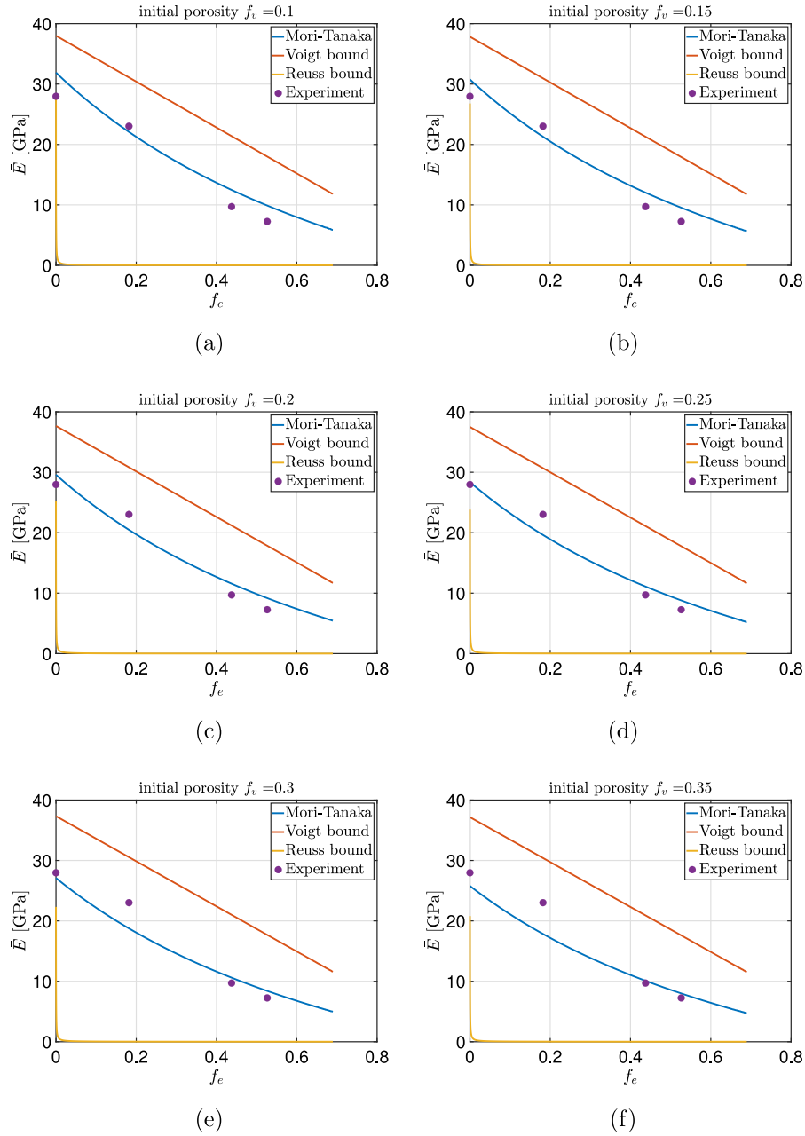
Fig. 8. Evaluation of the Young's modulus \bar{E} of the composite as a function of the volume fraction f_e , for different values of the porosity f_v . The inclusions are modeled as spherical.
