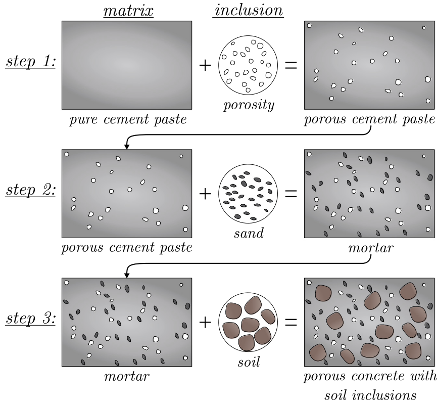
Fig. 3. Chart of the three steps of the homogenization procedure.
