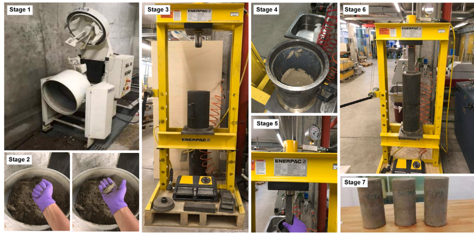
Fig. 6. Stage 1: Rotation panel mixer used to make composite specimens. Stage 2: Check of workability level by a visual examination of the mixture, according to the protocol used by practitioners. Stage 3: Equipment for molding, compacting and demolding specimens of step 3. Stage 4: Inserting of the fresh mixture of step 3 within a steel formwork by setting five layers of homogeneous thick one above the other. Stage 5: Compacting each layer with a given stress level. Stage 6: Demolding specimens of step 3. Stage 7: Visual examination of specimens before curing.
