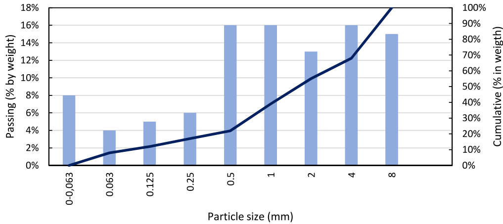
Fig. 5. Particle size curve of excavated soil used to make specimens of step 3.
