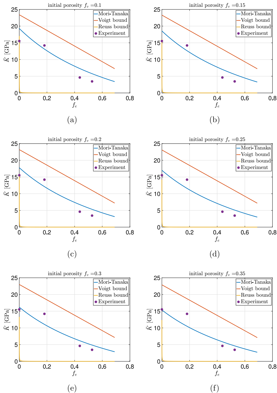
Fig. 10. Evaluation of the bulk modulus \bar{K} of the composite as a function of the volume fraction f_e , for different values of the porosity f_v . The inclusions are modeled as spherical.
