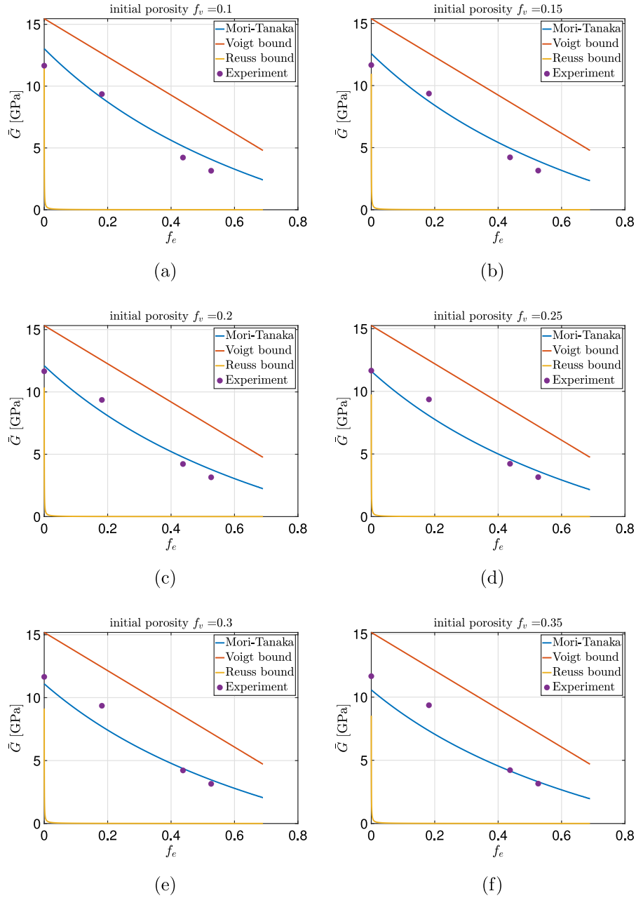
Fig. 9. Evaluation of the shear modulus \bar{G} of the composite as a function of the volume fraction f_e , for different values of the porosity f_v . The inclusions are modeled as spherical.
