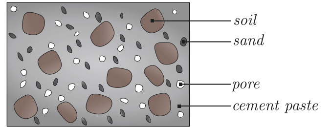
Fig. 2. Shot-earth can be schematized as a porous concrete with soil inclusions.
