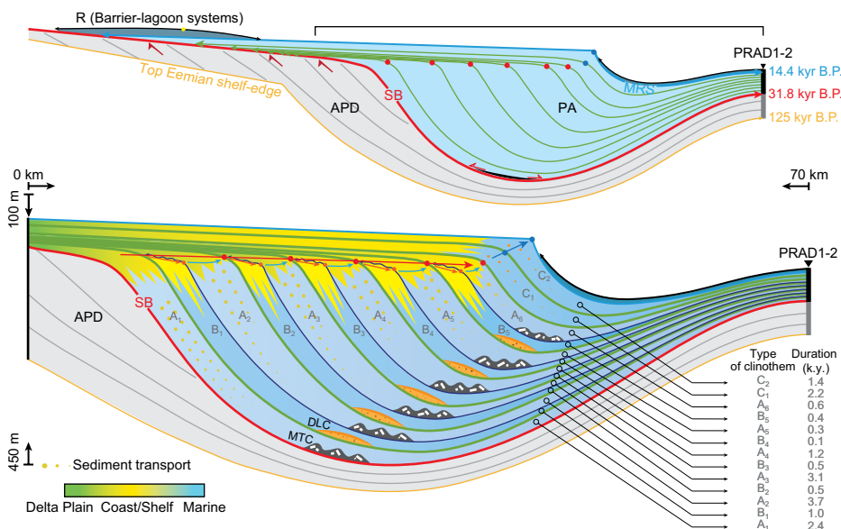
Figure 4. Top: Architecture of Po River (Italy) lowstand wedge characterized by progradational-aggradational (PA) cliniothems between sequence boundary (SB) and maximum regressive surface (MRS). Paleo-shelf edge at Eemian time is given for reference along with aggradational-progradational-degradational (APD) set preceding PA set. Atop PA set, lagoonal deposits (R) mark major back-step of paralic environments (Amorosi et al., 2016). Bottom: Detail of lowstand systems tract (PA set) recording millennial- to centennial-scale perturbations with alternating type A (slightly aggradational topset highlighted by light blue arrow and mass-transport complexes [MTCs] in basin) and type B (degradational topset highlighted by orange arrow and distributary channel-lobe complexes [DLCs] in bottomset). Type C develops during initial phase of post-Last Glacial Maximum sea-level rise and heralds greatest topset aggradation.
