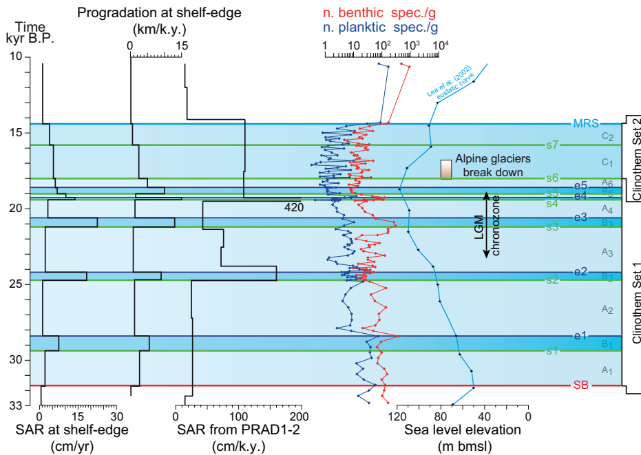
Figure 3. Sediment progradation and accumulation rates derived for each cliniothem at shelf-edge and in PRAD1-2 borehole, Po River (Italy) lowstand wedge, with foraminifera abundance (blue, planktic; red benthic; n.—number; spec.—specimens) and eustatic curve (meters below mean sea level [m bmsl]; Lea et al., 2002). Vertical scale is in time (calibrated kyr B.P.). Chronology is based on 14 C dating, integrated with tephrochronology, stable isotopes, and biostratigraphy at continuous-recovery borehole PRAD1-2. Type B cliniothems (darker stripes) develop at centennial-scale and with higher sediment accumulation rates (SAR, up to 22.4 cm/yr) compared to millennial-scale type A and type C cliniothems (lighter stripes). Red line is sequence boundary (SB) at base of Po River lowstand wedge; green lines (s) mark surfaces on top of type A and type C cliniothems whereas blue lines (e) are on top of type B cliniothems; light blue line is maximum regression surface (MRS) on top of younger type C2 cliniothem (cliniothems are numbered from older to younger). Cliniothem set 1 spans Last Glacial Maximum (LGM) sea-level fall and lowstand while cliniothem set 2 developed during initial phase of post-LGM sea-level rise. Brown box highlights timing of major retreat of Alpine glaciers (Monegato et al., 2007).
