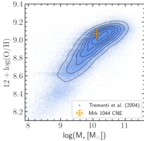
Fig. 14. Mrk 1044’s gas-phase metallicity relative to the mass–metallicity relation from Tremonti et al. (2004). Compared to star-forming galaxies with a similar stellar mass, Mrk 1044’s CNE has a higher metallicity by 0.11 dex.
