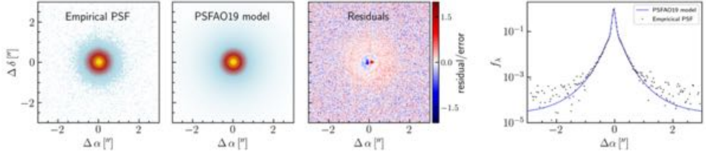
Fig. 3. Fitting the MUSE NFM-AO PSF. From left to right , the panels show the empirical PSF for the broad H \beta line extracted as described in Sect. 2.4.1, the corresponding PSFAO19 model, and the residual flux map. The rightmost panel shows the cross section of the PSF at the QSO position and fixed \delta . While the turbulent halo of the AO-induced PSF is well reproduced by the PSFAO19 model, the systematic errors near the center are significant compared to the relatively faint host signal.
