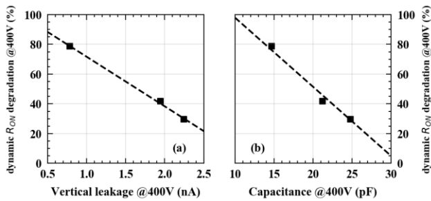
Fig. 5. (a) Correlation between Vertical leakage and dynamic R_{ON} degradation measured at V_{DS, stress} = 400 V. Higher Leakage (i.e., reduced buffer isolation) corresponds to lower dynamic R_{ON} coherently with a reduced net acceptor concentration in the Buffer layer. (b) Correlation between Capacitance and dynamic R_{ON} measured at V_{DS, stress} = 400 V. Higher Capacitance corresponds to lower dynamic R_{ON} coherently with a reduced net acceptor concentration in the buffer layer (i.e., reduced 2-DEG depletion).
