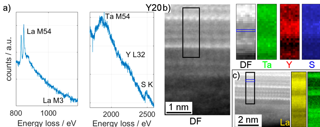
Figure 5. EELS analysis of an NT from sample Y20. (a) Spectra of the La M-edge as well as the Ta M-, Y L-, and S K-edges are taken from regions marked blue in the dark field (DF) images in b and c, respectively. (b) Ta and Y are spatially separated between the different layers recognized in the DF image. (c) La spectrum image obtained on the same NT showing enrichment of La in the two layers of MS.
