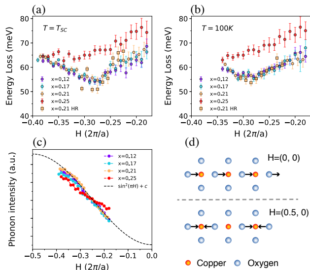
FIG. 3. Momentum dependent energy and intensity of the BS phonon mode. (a)&(b) Show the phonon energy dispersion and softening in the vicinity of \mathbf{Q}_{CDW} at (a) T = T_{SC} and (b) T = 100\text{ K} . Circles and squares represent data from Fig. 2 ( \Delta E = 55\text{ meV} ) and Fig. 1 ( \Delta E = 30\text{ meV} ), respectively. (c) Plots the integrated intensity of the BS phonon mode in the [40, 120]\text{ meV} energy window after subtracting elastic peak. The dashed line represents the \sin^2(\pi H) + \text{const.} fit to LSCO21. (d) Illustration of the oxygen atom displacements involved in the BS mode at H = (0, 0) and (0.5, 0) .
