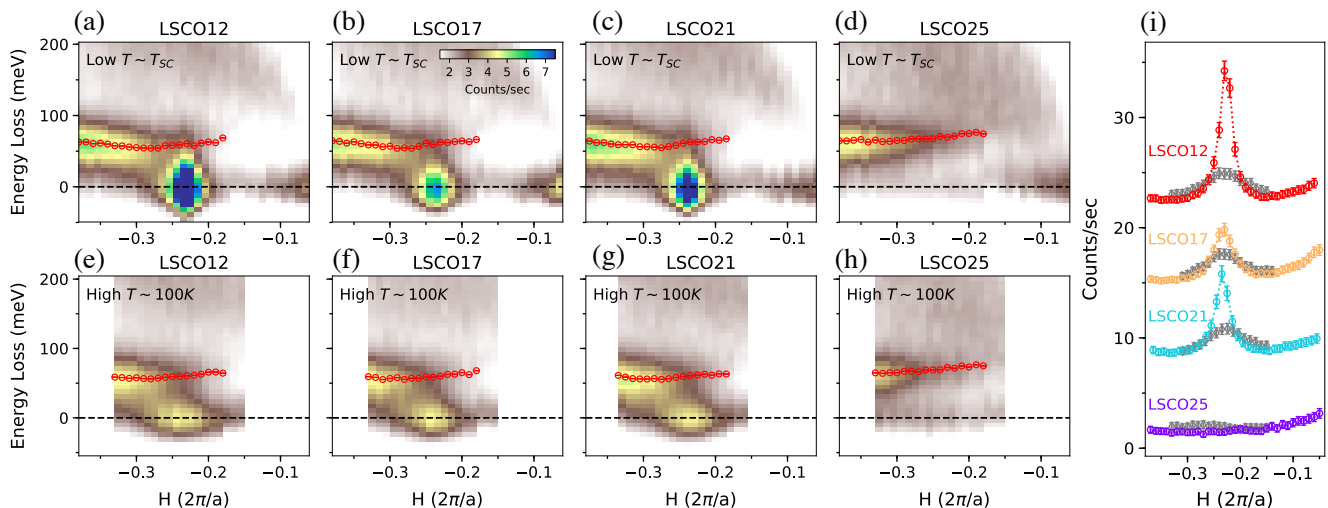
FIG. 2. Doping and temperature evolution. (a)-(d) show ( \Delta E = 55 meV) RIXS maps of LSCO_n ( n = 12, 17, 21, 25 ) at their superconducting transition temperature T_{SC} , where the CDW is strongest. All maps share the same colorscale inset in panel (b). Red circles represent the BS phonon energy. (e)-(h) The same measurement for T = 100 K. (i) Comparison of integrated intensity in the \pm 20 meV energy window. Data from panels (a)-(d) at T = T_{SC} are represented in color; data at T = 100 K from panels (e)-(h) are plotted in gray.
