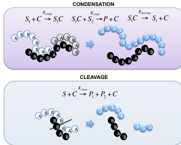
Figure 1: A schematic representation of the two allowed reactions. TOP: Condensation reaction. The white and the grey chains stand for the substrates, the black chain represents the catalyst and the blue chain stands for the product. The reaction occurs in two steps, the formation of a temporary molecular complex and the release of the product. BOTTOM: Cleavage reaction. The white chain represents the substrate, the black chain stands for the catalyst and the blue chains are the two products of the reaction.
