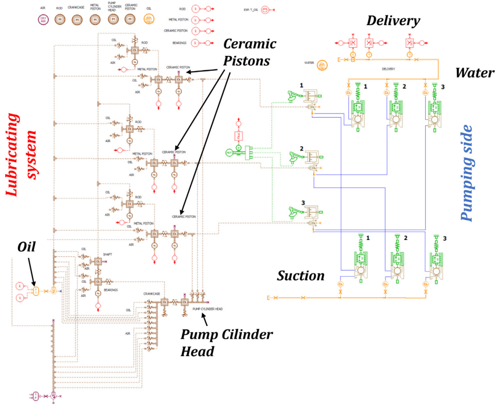
Fig. 4. Lumped parameter model, layout of the whole pump.
