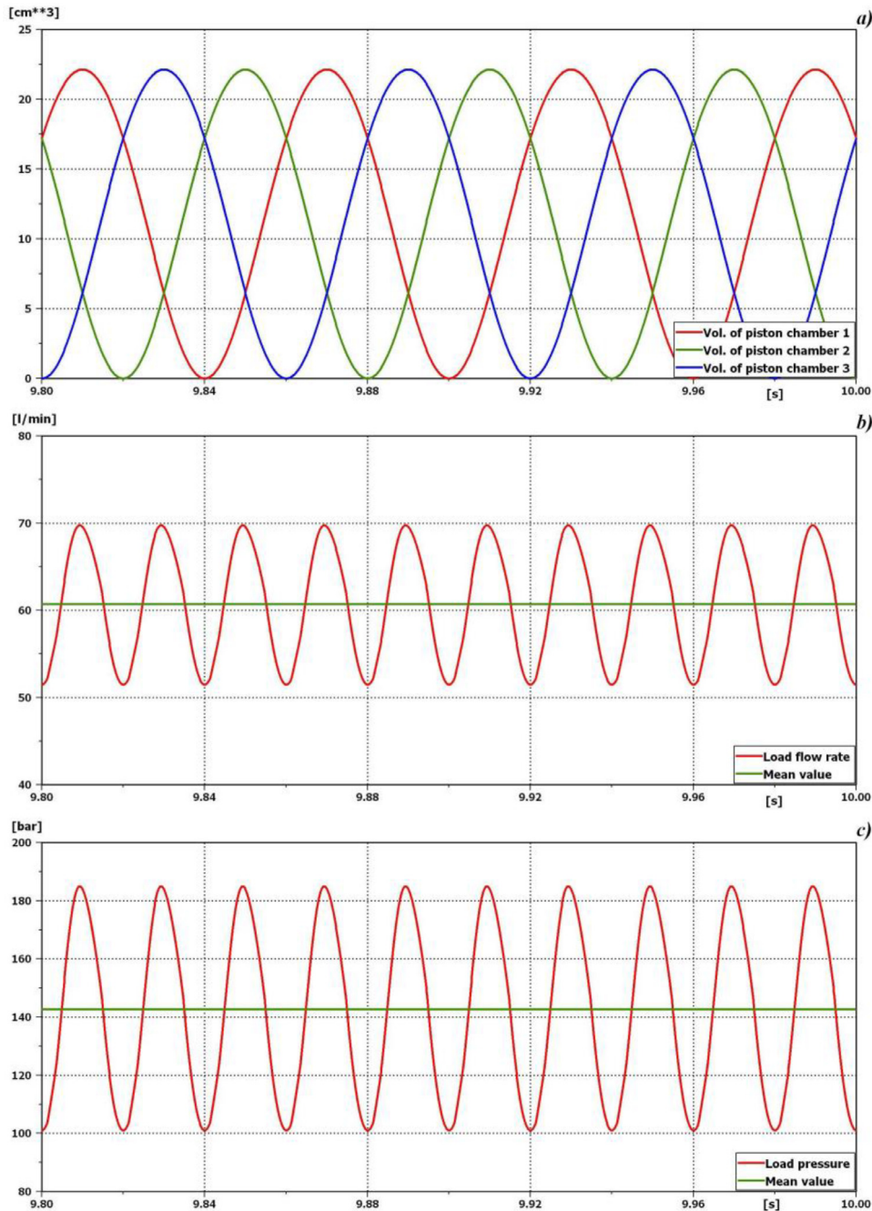
Fig. 6. Pumping side analysis: a) Phasing of piston chamber volume; b) load flow rate; c) load pressure.
