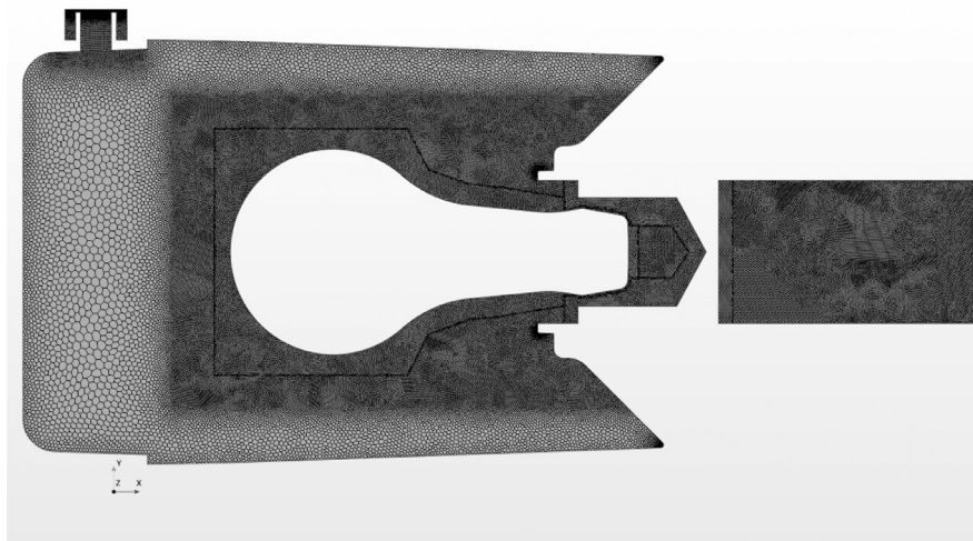
Fig. 2. Computational domain of the pump.
