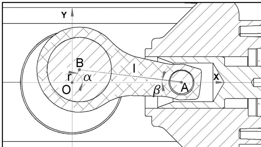
Fig. 3. Crank-rod mechanism, reference system.2.2 Friction model.
