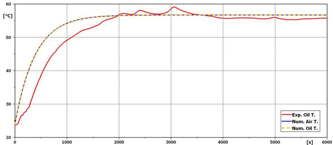
Fig. 8. Comparison between measured and calculated oil temperature.
