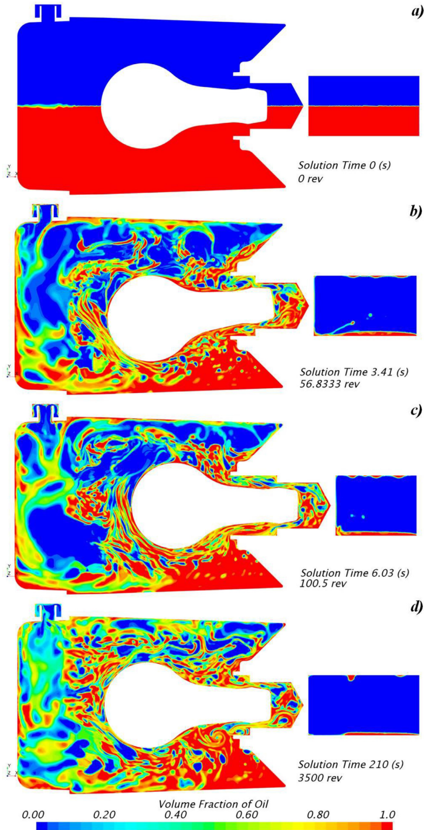
Fig. 5. Volume fraction of oil in the crankcase, referred to a) initial condition; b) after 3.41 s c) after 6.03 s; d) after 210 s.
