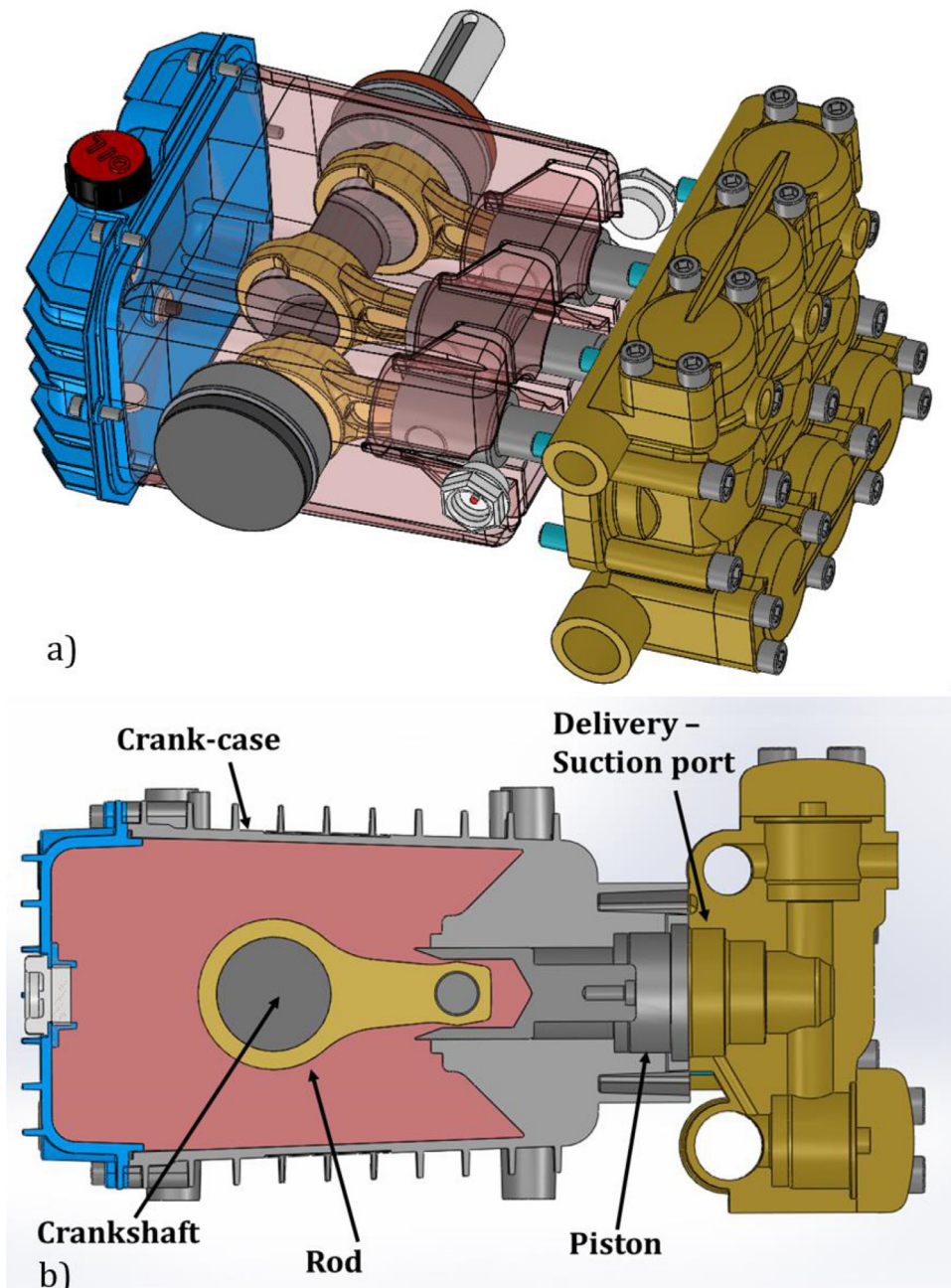
Fig. 1. (a) Geometry of the piston water pump analysed and (b) vertical section through the central piston.
