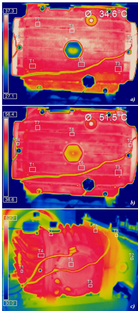
Fig. 7. Thermographic analysis: a) crankcase cover after a few seconds; b) crankcase cover in steady-state condition; c) whole pump in steady-state condition.
