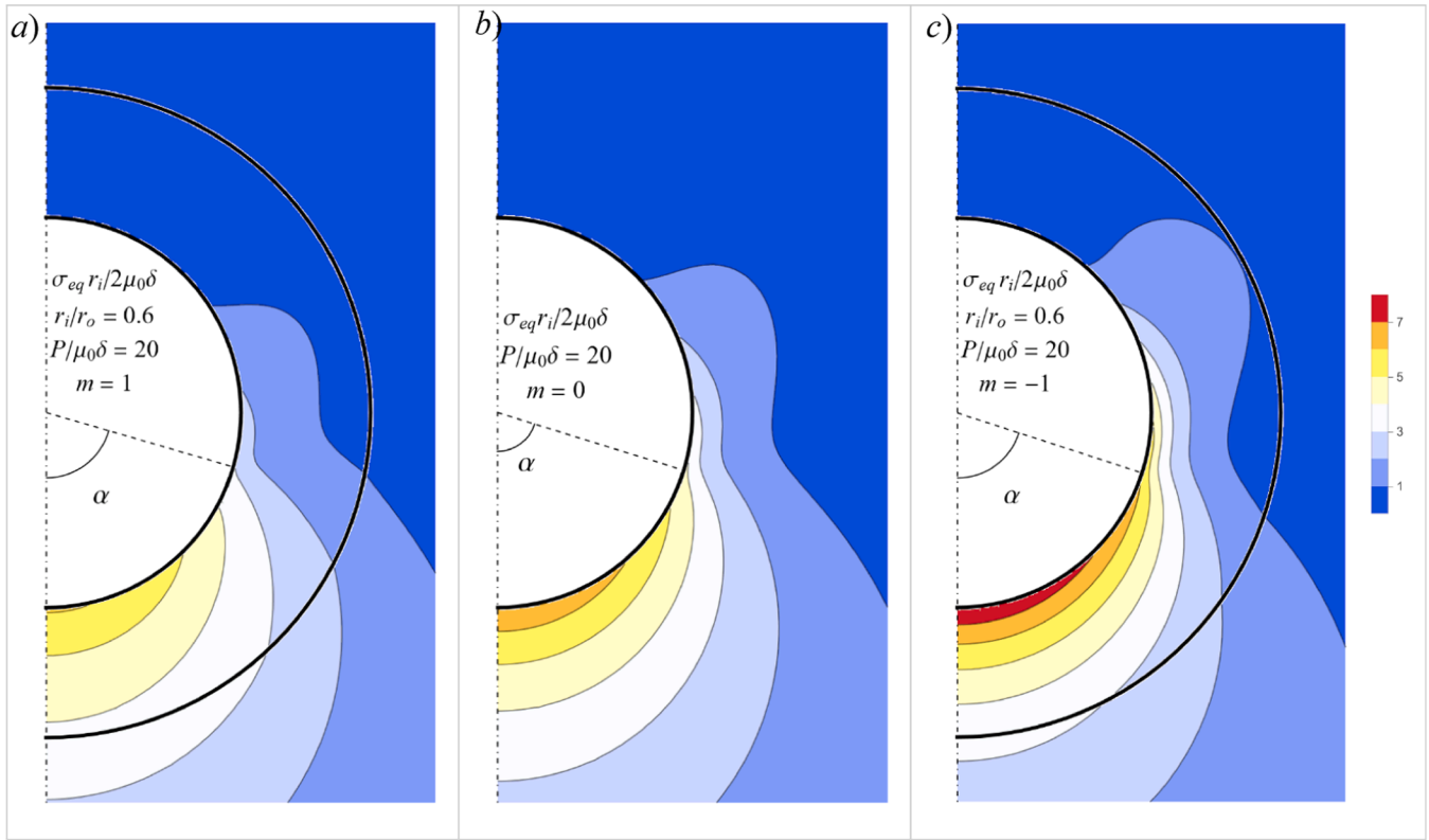
Fig. 12. Analytical distributions of the normalized von Mises equivalent stress \sigma_{eq} r_i / (2\mu_0\delta) under plane strain condition in the FGM ring with aspect ratio r_i/r_o = 0.6 and the isotropic elastic plane, under the pin load P/(\mu_0\delta) = 20 , for positive ( m = 1 ) (a), null ( m = 0 ) (b), and negative ( m = -1 ) (c) grading indices.
