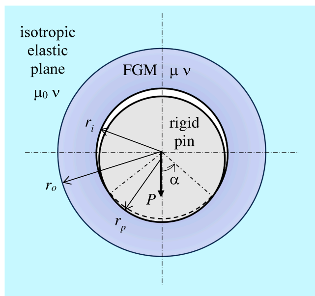
Fig. 1. Loaded rigid pin in a hole in an isotropic elastic plane with a FGM annular reinforcement.
