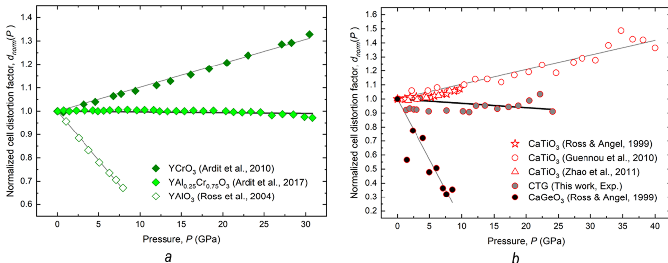
Figure 7. Normalized cell distortion factor with pressure, d_{\text{norm}}(P) , for YM^{3+}O_3 (a) and CaB^{4+}O_3 (b) orthorhombic perovskites, as derived from X-ray diffraction experiments. The solid lines are linear fits to the data. In panel (a), data for the isotypic series YM^{3+}O_3 ( M = \text{Cr} and \text{Al} ) are from 1,50,51 . In panel (b), data for the isotypic series CaB^{4+}O_3 ( B = \text{Ti} and \text{Ge} ) are from this work and 11,45,46 .
