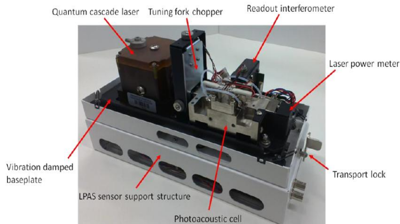
Figure 1–Layout of the LPAS module.
