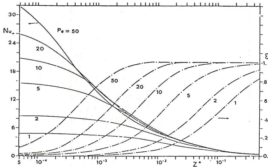
Fig.7 - Nusselt number and performance ratio vs. Z ( Z \geq 0 )
