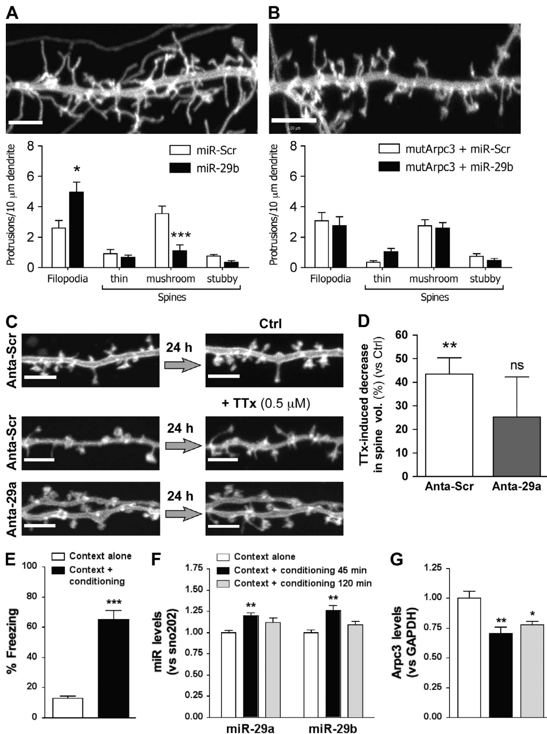
Figure 7. miR-29a and -29b regulate sensitivity to neuroplastic changes. (A and B) Primary cultures of hippocampal neurons at 9 DIV were transfected with EGFP-MEM ± Arpc3 in which the miR-29 seed region contained two point mutations (mutArpc3) plus siRNA oligonucleotides. Effects on neuronal structure were investigated at 14–15 DIV using confocal microscopy. Data are representative images plus graphs demonstrating the mean ± SEM number of protrusions for miR-Scr and miR-29b for EGFP-MEM alone (A) or EGFP-MEM plus mutArpc3 (B). (A) As demonstrated previously, miR-29b enhances the number of filopodia ( P = 0.01 ) and reduces the number of mushroom spines ( P < 0.001 ; n = 12 ). (B) miR-29b did not alter dendritic morphology in neurons expressing mutArpc3 ( n = 12 ). (C–E) miR-29a antagonist reduces spine volume changes induced by TTx. Dendritic regions of hippocampal neurons cotransfected with EGFP-MEM plus 50 nM miR-Scr or miR-29a antagonist were imaged via confocal microscopy at 14 DIV and then again after 24 h in the presence or absence of 0.5 μM TTx. Changes in spine volume were calculated from 3D volume-rendered images. (C) Representative dendritic images for Scr antagonist and miR-29a antagonist neurons before and after a 24-h period under control (Ctrl) conditions or in neurons treated with TTx. Note the loss of spine structure in Scr antagonist after 24 h in the presence of TTx (middle). (D) Expression of miR-29a antagonist did not alter spine volume measured at 14 DIV (data from 200 and 170 spines; not depicted). Treatment with TTx for 24 h reduced spine volume in Scr antagonist neurons by 43.5 \pm 6.9\%
