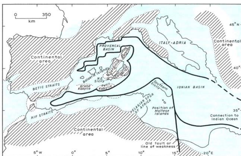
Fig. 3: Structural setting of the Mediterranean area during the Oligocene (from Pedley et al., 2002).
