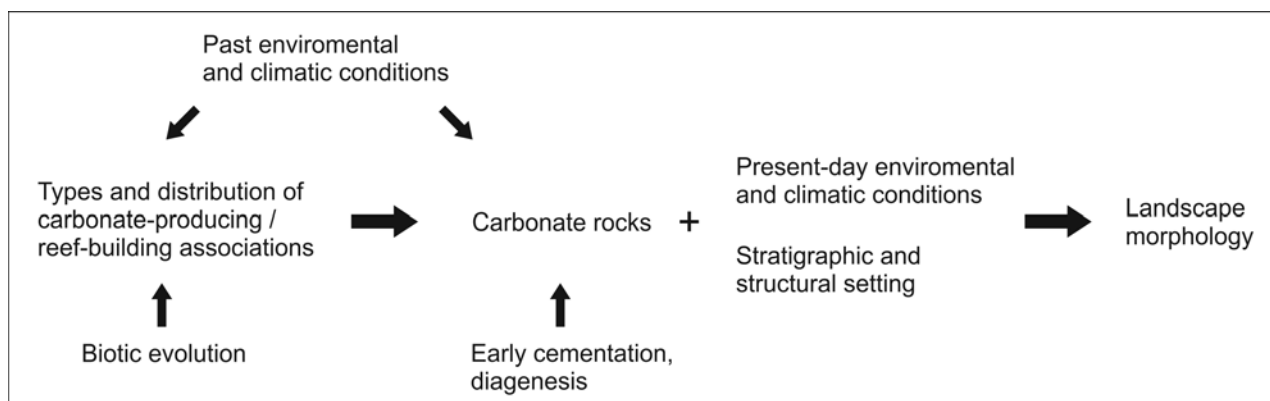
Fig. 11: Relations among biosphere, carbonate production and landscape evolution.
