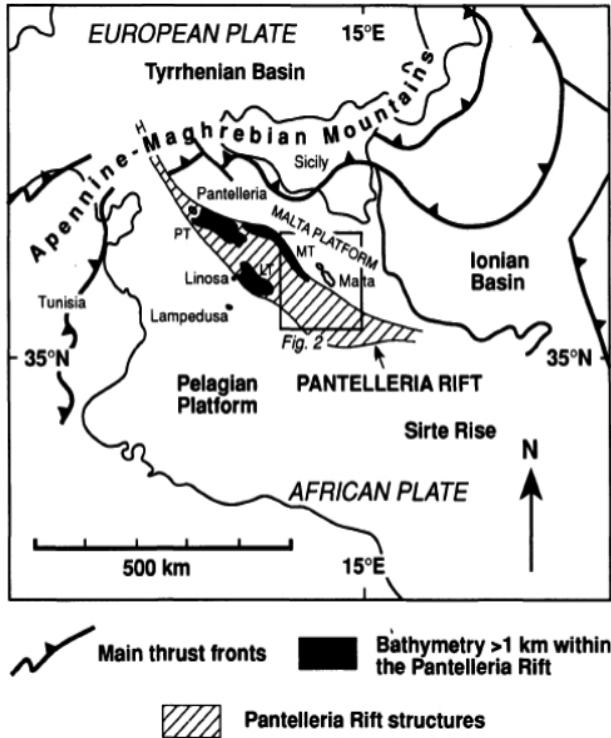
Fig. 5: Location of the Maltese graben system within the central Mediterranean. PT, Pantelleria Trough; LT, Linosa Trough; MT, Malta Trough (from Dart et al., 1993).
