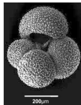
Fig. 16: A Globigerina specimen showing the aggregation of spheroidal chambers.
