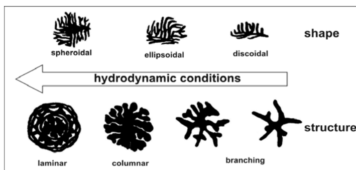
Fig. 15: Relations among rhodoliths shape and structure and hydrodynamic conditions (modified from Bosence, 1991).
