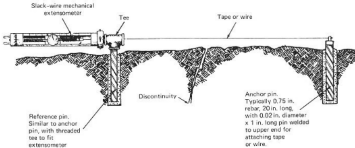
Fig. 1: The TE technique uses a steel wire and pins where the instrument is anchored.
