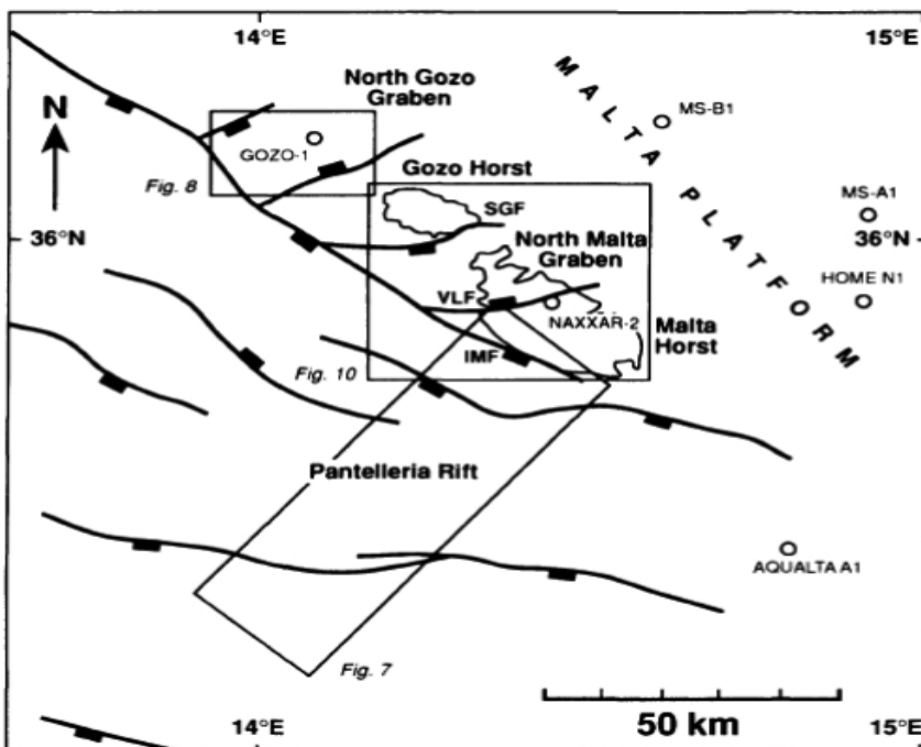
Fig. 6: Principal structures of the Maltese graben system. SGF, South Gozo fault; VLF, Victoria Lines fault; IMF, Ii Maghlaq fault (from Dart et al., 1993).
