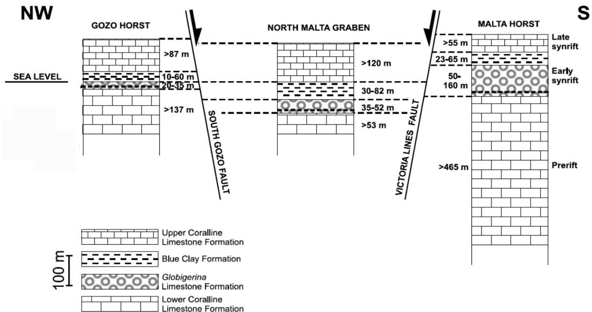
Fig. 7: Stratigraphic correlation between the structural elements of the North Malta Graben system. The Gozo and Malta horsts are separated by the North Malta Graben, which is bound by the south Gozo fault and the Victoria Lines fault to the north and south, respectively (modified from Putz-Perrier and Sanderstone, 2010).
