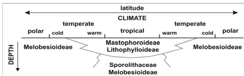
Fig. 12: Distribution of coralline algae subfamilies in relation to climate and depth (from Aguirre et al., 2000).
