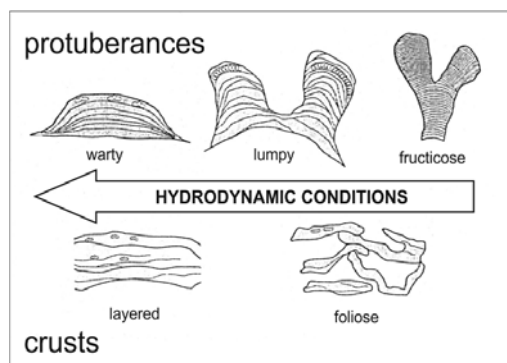
Fig. 13: Relations between coralline algae growth forms and hydrodynamic conditions (modified from Nebelsick and Bassi, 2000).
