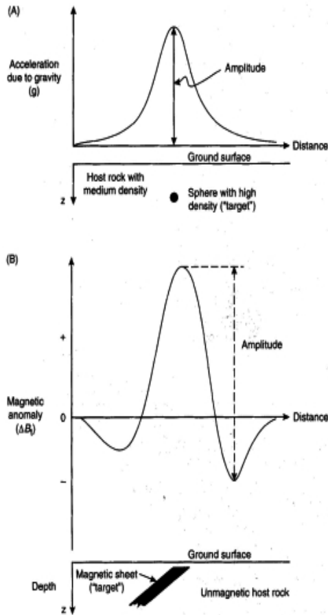
Fig. 1: A) Gravimetric anomaly due to the presence of a sphere with high density in the ground; B) Magnetic anomaly due to the presence of a magnetic sheet below the ground surface.
