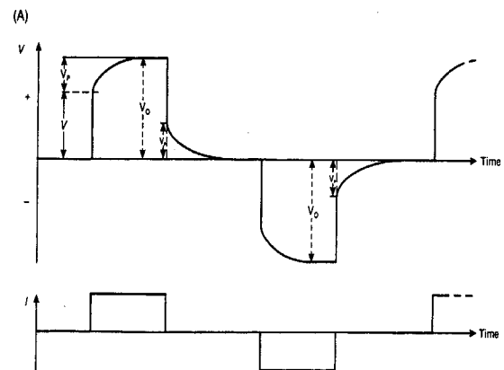
Fig. 3: Scheme of V and I variations with time in a polarizable medium.
