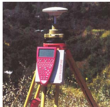
Fig. 1: The Global Positioning System (from Hofmann-Wellenhof et al., 2001).
