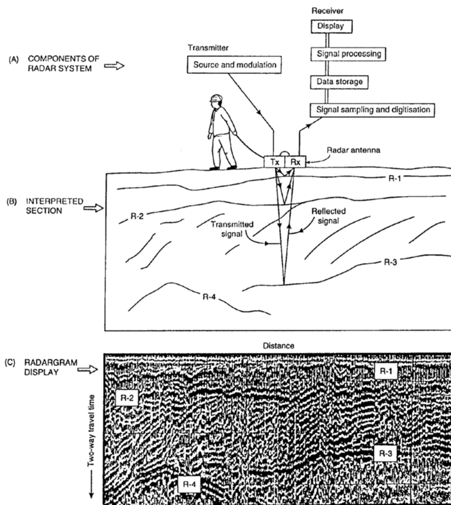
Fig. 2: Simplified GPR scheme (from Davis and Annan, 1989).
