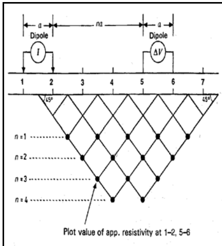
Fig. 1: Scheme of resistivity pseudosection (Dipole-Dipole electrodes configuration).
