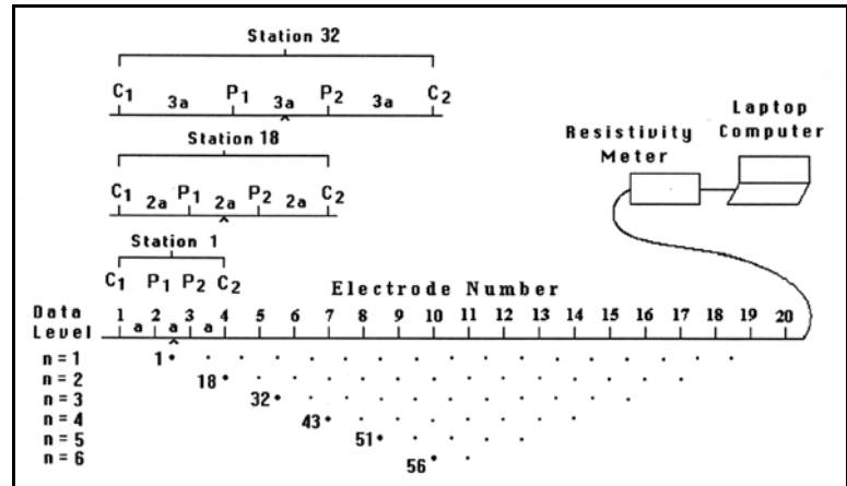
Fig. 2: Sequence of electrodes combinations to acquire a resistivity pseudosection (Wenner array).
