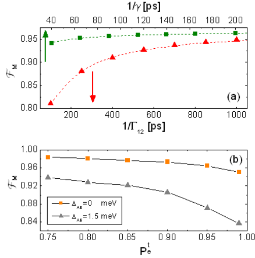
Fig. 4. (Color online) (a) Dependence of the maximum fitness function \mathcal{F}_M on the 1/\gamma (upper axis, green squares) and \Gamma_{21} (lower axis, red triangles), being \gamma and \Gamma_{12} the dephasing and non-radiative relaxation rates, respectively; g^{AB} = 1 and \Delta_{AB} = 1.25 meV. The green (red) dotted line represents the best fit of \mathcal{F}_M linear (quadratic) in \gamma ( \Gamma_{21} ). (b) \mathcal{F}_M as a function of the threshold P_e^t in the photon-emission probability for g_{AB} = 1 , with \Delta_{AB} = 0 and 1.5 meV.
