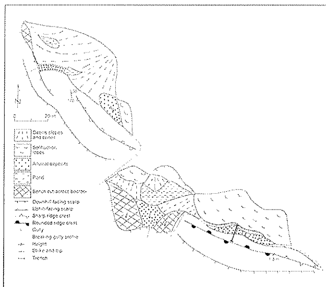
Fig. 6: Detailed geomorphological map of the trenched sackung features. This sketch was produced by direct mapping on graph paper in the field using a laser distancimeter and compass.
