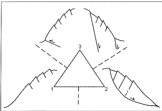
Fig. 1: Ternary diagram illustrating three end-members of slopes with sackung features: (1) Sackung failure planes that grade downwards into a continuous deformation. (2) Antithetic sackung failures connected to the sliding surface of a deep-seated landslide. These two extremes may represent a temporal gradation. (3) Sackung failures that correspond to secondary ruptures associated to active faults.
