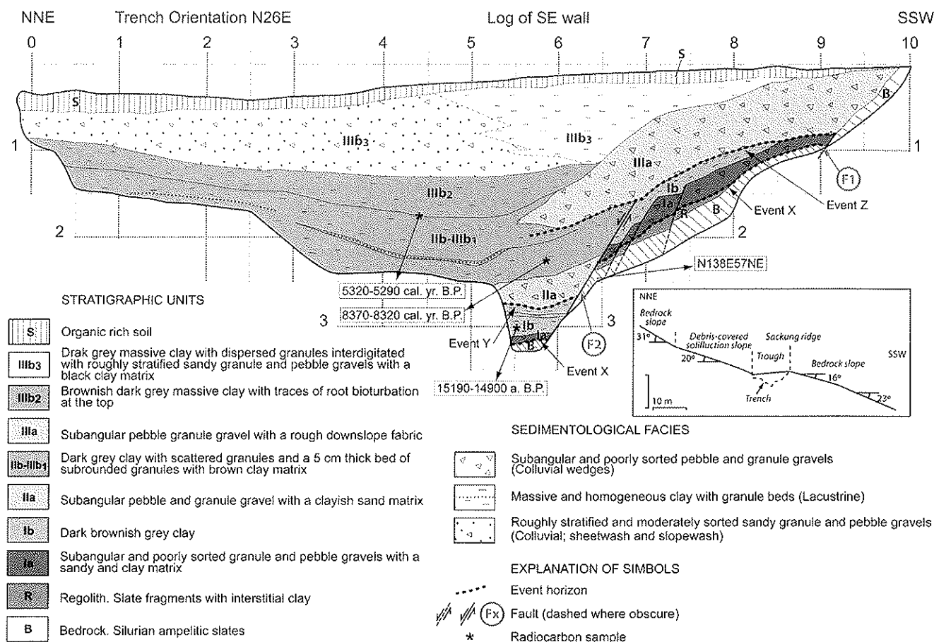
Fig. 8: Log of the SE wall of the trench and topographic profile of the slope at the trench site. Calendar ages correspond to ranges at 1σ. The location of the trench is shown in figures 3 and 6.
