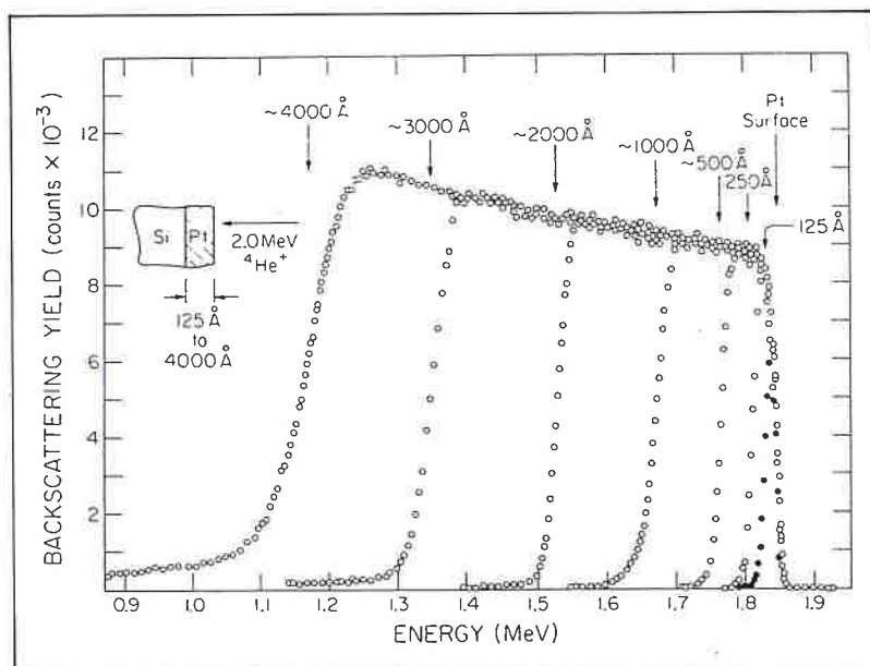
Figure 8. RBS Spectrum. Many layer target ( 12.5 \leq t \leq 400 nm) 5 .
