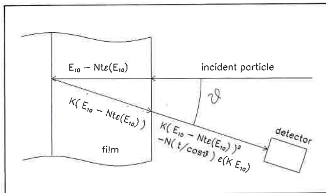
Figure 7. The incident particles with energy E_{i0} penetrate into a sample of thickness t ; backscattered towards the detector, their energy is reduced by a factor K and they cross again a thickness t of material.
