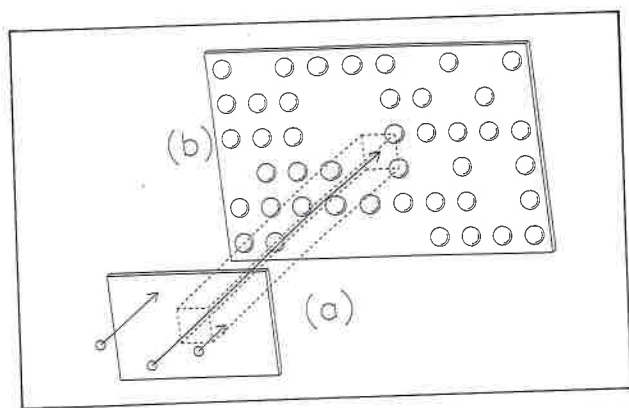
Figure 3. Scheme of a beam of particles colliding on a target, constituted by particles arranged in a bi-dimensional array (section b). The dotted parallelogram represents the active volume of a beam particle (e.g., the region in which it can interact with a target particle).
