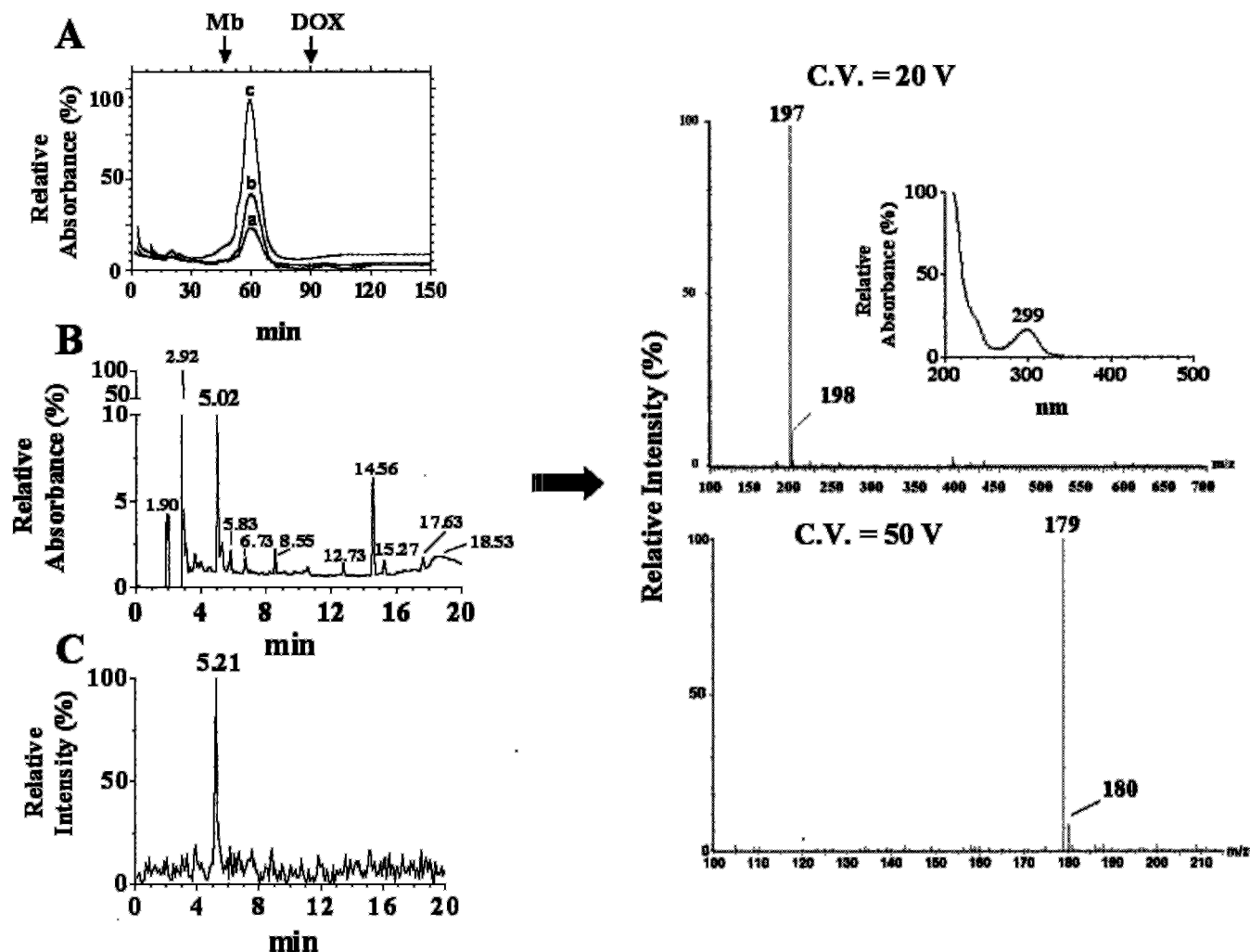
FIG. 5. Gel permeation, HPLC, and HPLC/ESI(+)-MS of DOX/Mb IV ultrafiltrates. Incubations (1 ml final volume) contained DOX (100–500 \mu\text{M} ) and equimolar Mb III , always reacted with a 2-fold excess of H 2 O 2 . After 10 min, reactions mixtures were added with catalase (2600 units) and ultrafiltered. A shows gel permeation of ultrafiltrates derived from Mb IV -degraded DOX (100 \mu\text{M} (line a ), 200 \mu\text{M} (line b ), or 500 \mu\text{M} (line c )); the upper arrows indicate the retention times of Mb III or DOX standards chromatographed under comparable conditions. B shows HPLC of gel-filtered fraction c in A , and C shows the corresponding HPLC/ESI(+)-MS chromatogram. ESI(+)-MS of the HPLC fraction eluted at 5.21 min was carried out at C.V. = 20 or 50 V; the inset in the upper panel shows the UV spectrum associated with the HPLC fraction eluted at 5.02 min.
