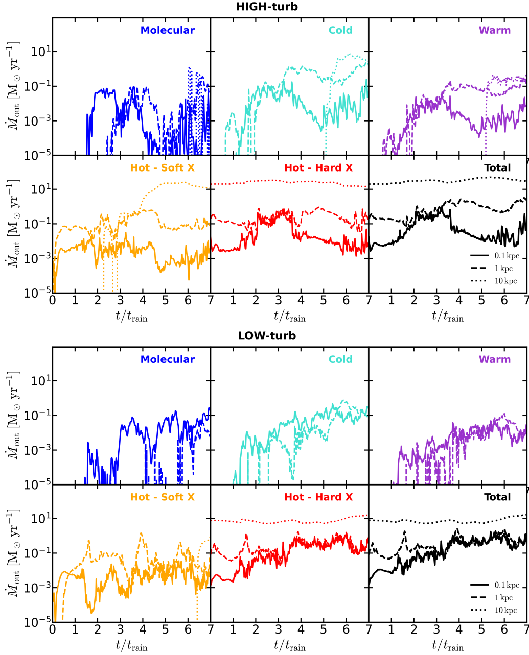
Fig. 7. Phase-separated mass outflow rates for the high-turb (top figure) and low-turb (bottom figure) runs as a function of time normalized to t/t_{rain} . Outflow is defined from gas with positive radial velocity, and each panel shows the corresponding \dot{M}_{out} for a given thermal phase: molecular, cold, warm, soft X-ray, hard X-ray, and the total (black lines). Solid, dashed, and dotted lines refer to r = 0.1, 1 , and 10 kpc, respectively. In the high-turb case, the molecular, cold and warm outflows are more extended and intermittent, consistent with stronger uplift and entrainment by the more disturbed medium. In the low-turb atmosphere, cool outflows are mostly confined to the inner kpc and are less intermittent, indicating a lower entrainment/uplifting due to the weaker turbulent stirring efficiency.
