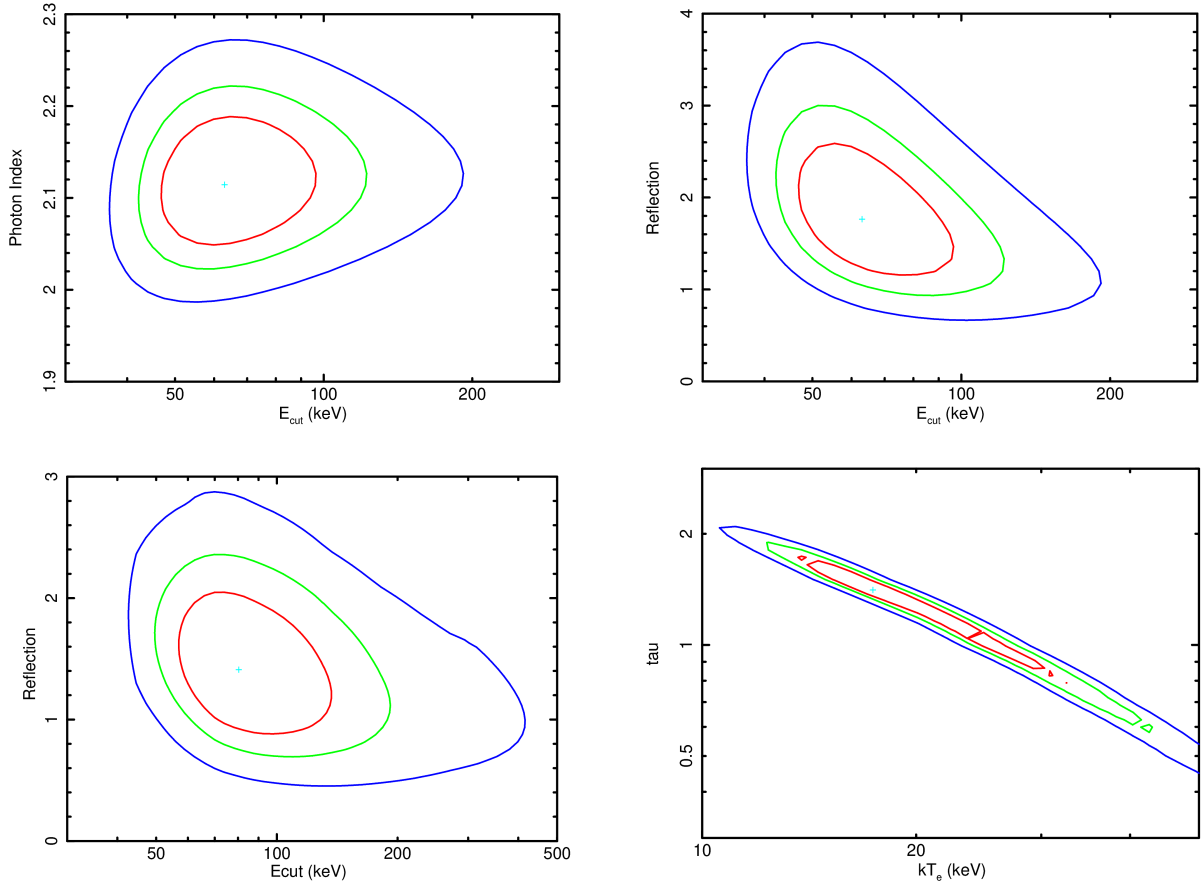
Fig. 2: Top row: Confidence contours for the PEX model, E_{\text{cut}} vs \Gamma (left) and E_{\text{cut}} vs R (right). Bottom row: Confidence contours for E_{\text{cut}} and R for the REFL model (left) and for kT_e and \tau for the CREFL model (right). The latter reveals a strong \tau - kT_e degeneracy: higher kT_e is compensated by lower \tau (and vice versa), to reproduce the same observed photon index \Gamma . Red, green, and blue contours show 68, 90, and 99% confidence levels, respectively.
