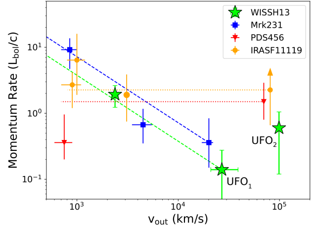
Fig. 8: Momentum rate vs. velocity of different outflow phases for WISSH13 (green stars), Mrk 231 (blue squares, Feruglio et al. 2015), PDS 456 (red triangles, Bischetti et al. 2019b) and IRASF 11119 (orange circles, Lanzuisi et al. 2024). Data points at v_{\text{out}} < 10^4 km/s refer to either molecular outflows (CO or OH detection) or to [OIII] and UV winds. Data points at v_{\text{out}} > 10^4 km/s refer to UFOs. Dotted horizontal lines show the evolution of a momentum-driven outflow in the case of PDS 456 and IRASF 11119, while dashed lines show the momentum boost expected for an energy-driven outflow in the case of Mrk 231 and WISSH13, if UFO 1 is considered.
