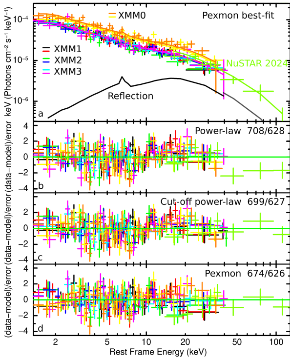
Fig. 1: Panel a shows the best-fit PEX model with the full XMM-Newton and NuSTAR data set. pn and MOS1+2 data are shown with different colors for each observation, identified by its name. The reflection-only component is shown in black. Panels b , c , and d , show residuals for the PL, CPL and PEX models, respectively. Residuals for the REFL and CREFL models are not shown for clarity, as they are indistinguishable from those in panel d . C-stat/d.o.f. is reported for each model. NuSTAR FPMA and FPMB data are co-added for plotting purposes only.
