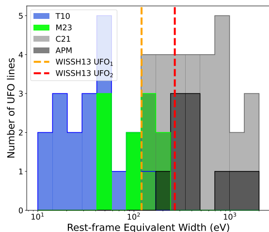
Fig. 4: Rest-frame equivalent widths for WISSH13 (orange and red dashed lines for \text{UFO}_1 and \text{UFO}_2 , respectively) compared with Seyferts at z < 0.1 in blue (Tombesi et al. 2010, T10), QSOs at z = 0.1 - 0.5 in green (Matzeu et al. 2023, M23) and lensed, high- z QSOs in gray (Chartas et al. 2021, C21, and references therein), including the multiple detections in APM 08279+5255 (Chartas et al. 2009), shown in black.
