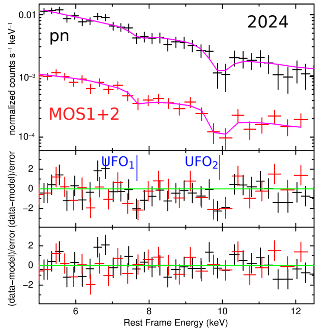
Fig. B.1: 2024 merged spectra: EPIC-pn (black) and MOS1+MOS2 (red). The best-fit model, including two absorption Gaussian lines, is shown in magenta. Middle: residuals without the two Gaussian absorption lines. Bottom: residuals with the two Gaussian absorption lines at the best-fit energy. The stack uses strictly flare-cleaned time intervals over the 2024 data set to ensure comparable background levels among the stacked spectra, and therefore has lower exposure time and counts (by 50%) than the full, jointly fitted 2024 spectra adopted in Section 3 .
