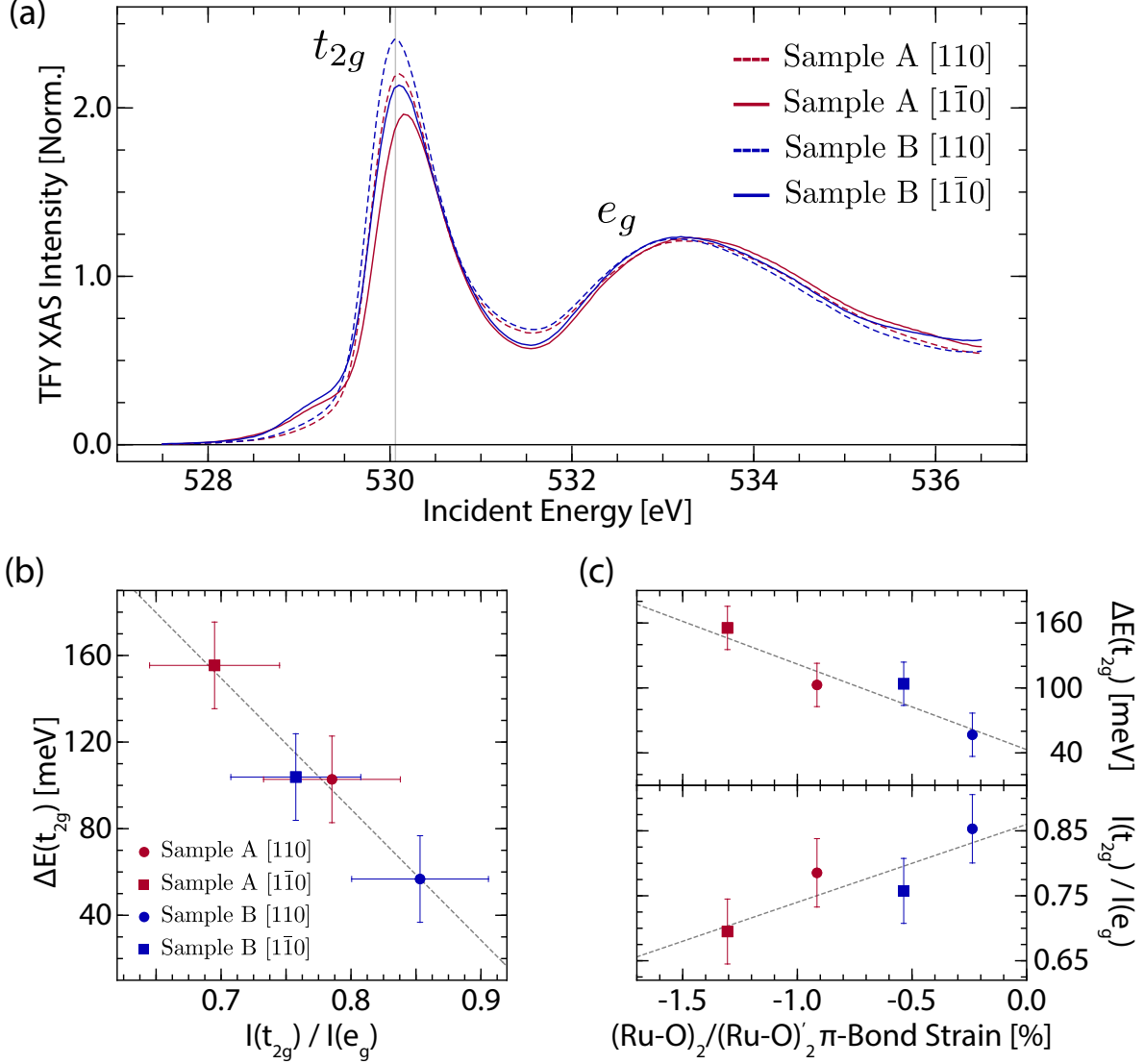
FIG. 3. (a) Comparison of the XAS spectra measured along the nominally equivalent [110] and [1\bar{1}0] directions in Samples A and B. Spectra have been normalized by the integrated \text{O}:2p \rightarrow \text{Ru}:e_g spectral weight. (b) Shift of the t_{2g} energy \Delta E(t_{2g}) plotted against the ratio I(t_{2g})/I(e_g) of the integrated t_{2g} and e_g transition spectral weights reveals a linear correlation. (c) Plots of \Delta E(t_{2g}) (top) and I(t_{2g})/I(e_g) (bottom) against the relative (\text{Ru-O})_2^{(l)} bond strain. The (\text{Ru-O})_2 bond length is used for \epsilon \parallel [1\bar{1}0] measurements (squares) and the (\text{Ru-O})'_2 bond is used for \epsilon \parallel [110] (circles) (see text and Ref. 6 for details). In (b,c), red/blue color denotes Sample A/B, respectively, and squares/circles indicate measurements with polarization along the [1\bar{1}0]/[110] directions, respectively.
