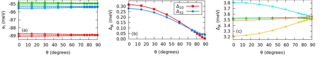
FIG. 2. (a) Lowest energy levels e_i ( i = 0, \dots, 3 ) and (b,c) corresponding energy gaps \Delta_{jk} \equiv e_j - e_k for holes in the reference quantum dot QD1. The color code for the energy gaps \Delta_{jk} between states belonging to different doublets, displayed in panel (c), is the following: \Delta_{21} (yellow), \Delta_{31} (salmon), \Delta_{20} (green), \Delta_{30} (cyan). The values of \omega_x , \omega_y , L_z , E_z , and B used in these calculations are reported in Table I (case C1) and in the table caption.
