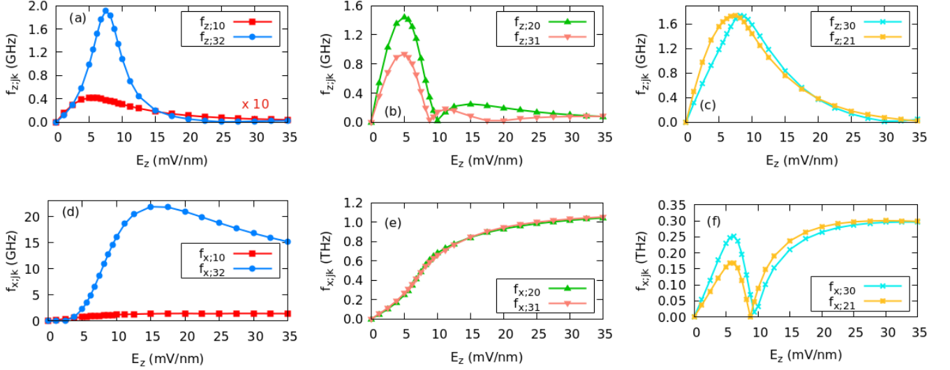
FIG. 6. Rabi frequencies (a,b,c) f_{z;jk} and (d,e,f) f_{x;jk} for QD1 as a function of the applied bias E_z , associated to a time-dependent field of amplitude \delta E = 1 mV/nm, oriented along the z and x directions, respectively. The values of \omega_x , \omega_y , L_z , \theta , and B used in these calculations are reported in Table I (case C4) and in the table caption.
