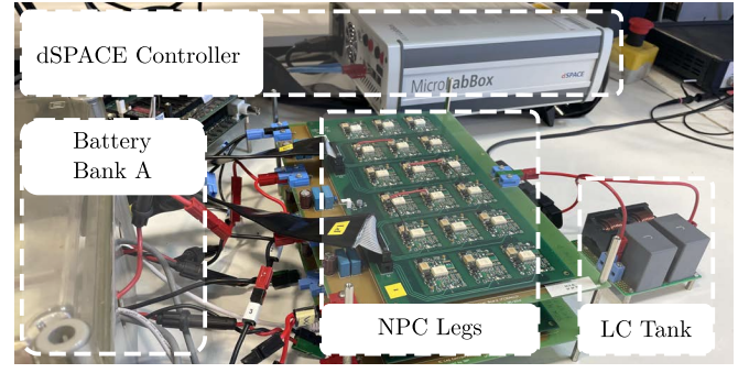
Fig. 8. Experimental hardware prototype.
