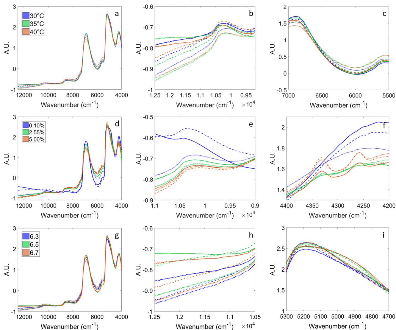
Fig. 2 SNV pretreated FT-NIR spectra of the beginning (solid lines), transition phase (dashed lines), and end (dotted lines) of milk renneting, averaged according to temperature (a–c), fat content (d–f), and pH (g–i).
