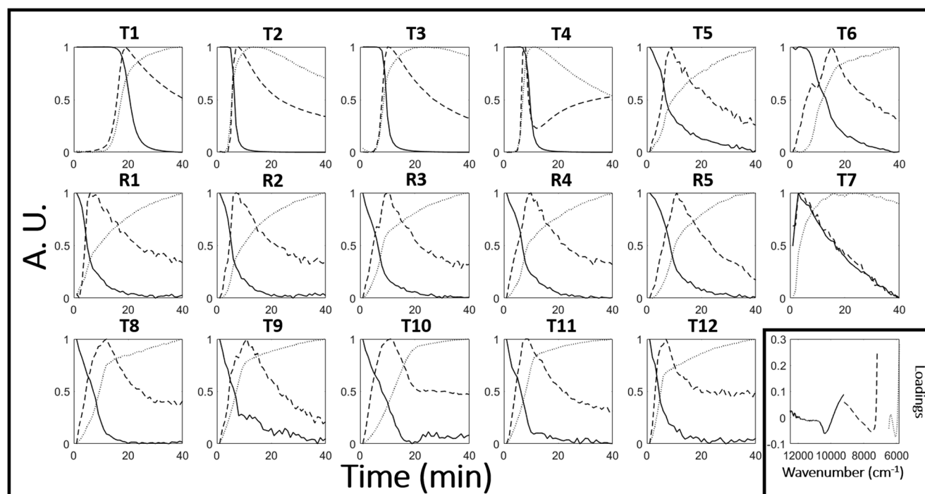
Fig. 3 Score profiles obtained from the i-PCA models calculated for each milk renneting trial. Solid lines, PC1 scores of the 12,500 to 9200 \text{cm}^{-1} range; dashed lines, PC2 scores of the 9199 to 7181 \text{cm}^{-1} range; dotted lines, PC1 scores of the 6463 to 5824 \text{cm}^{-1} range. The
