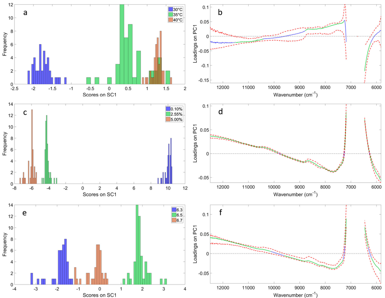
Fig. 4 Histograms of ASCA score frequency with projected residuals along SC1 for the different levels of experimental factors considered in the study of milk renneting: temperature (a), fat content (c), pH (e). The
