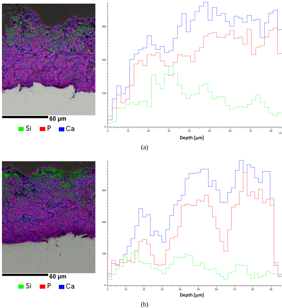
Figure 2.67: EDS maps and compositional profile of samples after in vitro test. a) sample immersed one week in SBF, (b) sample immersed two weeks in SBF
