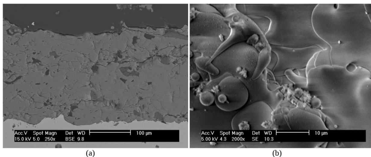
Figure 2.20: PS-HA coatings: (a) cross section (b) surface
