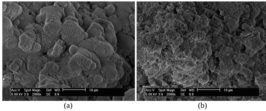
Figure 2.45: SEM images of the reference coatings after 14 days in SBF: (a) BG_Ca, (b) HA
