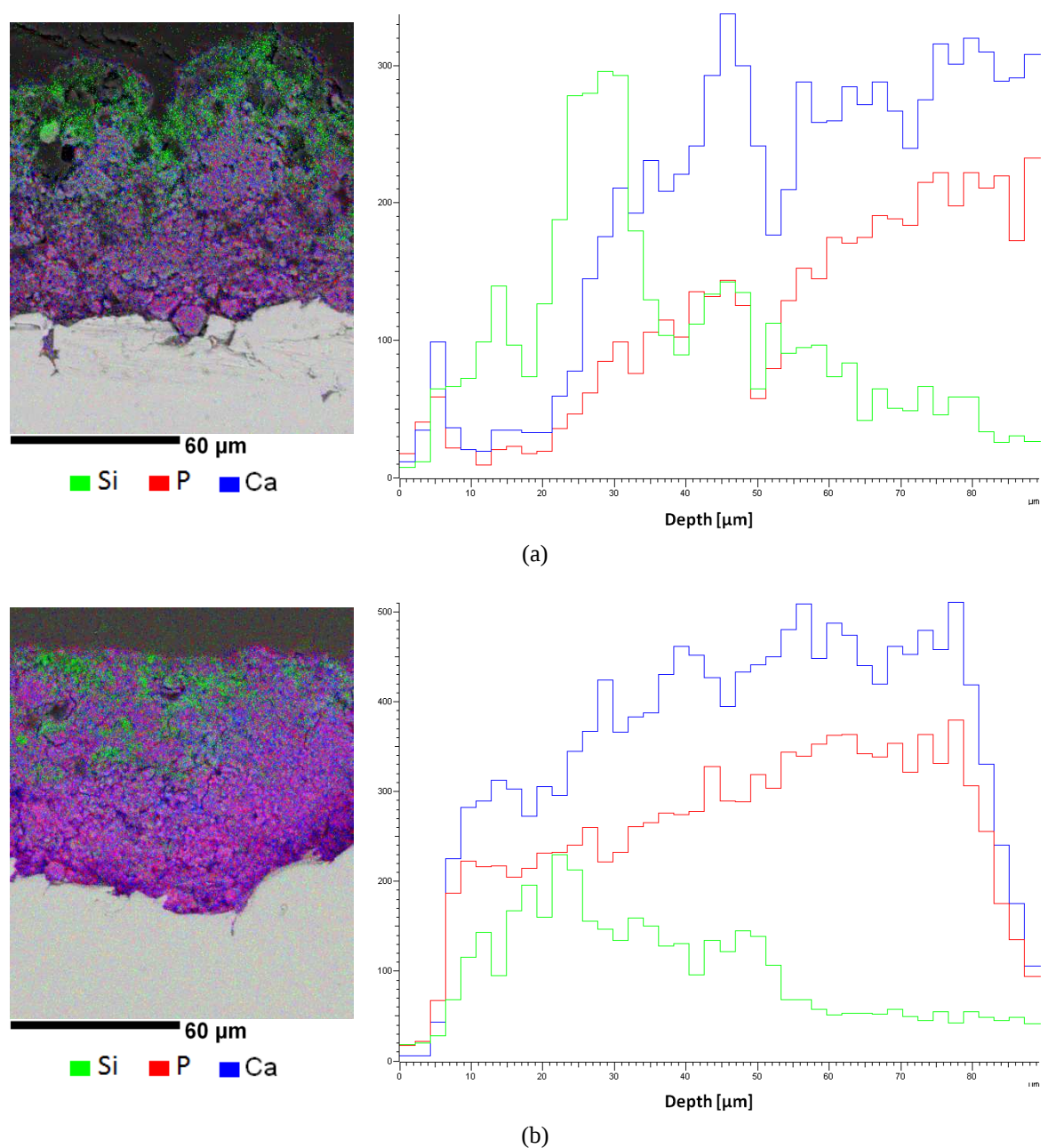
Figure 2.66: EDS maps and compositional profile of samples after in vitro test. (a) sample immersed one day in SBF, (b) sample immersed three days in SBF
