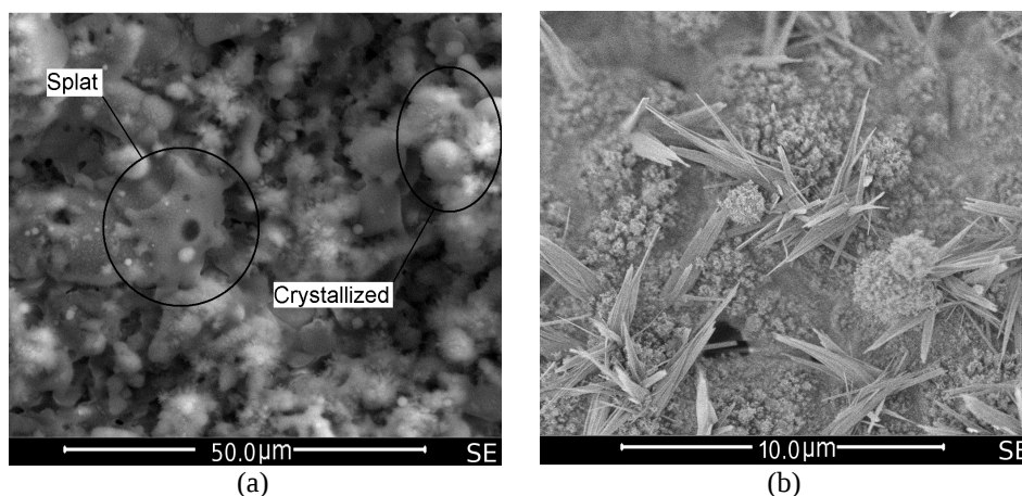
Figure 2.11: SEM micrographs (secondary electrons): the area representative of the surface morphology of the coatings (BGCa3 run) with molten splats and crystallized zones outlined (a); high magnification of a crystallized area (b) (note that the acicular morphology typical of \text{CaSiO}_3 can be observed as suggested in [144])
