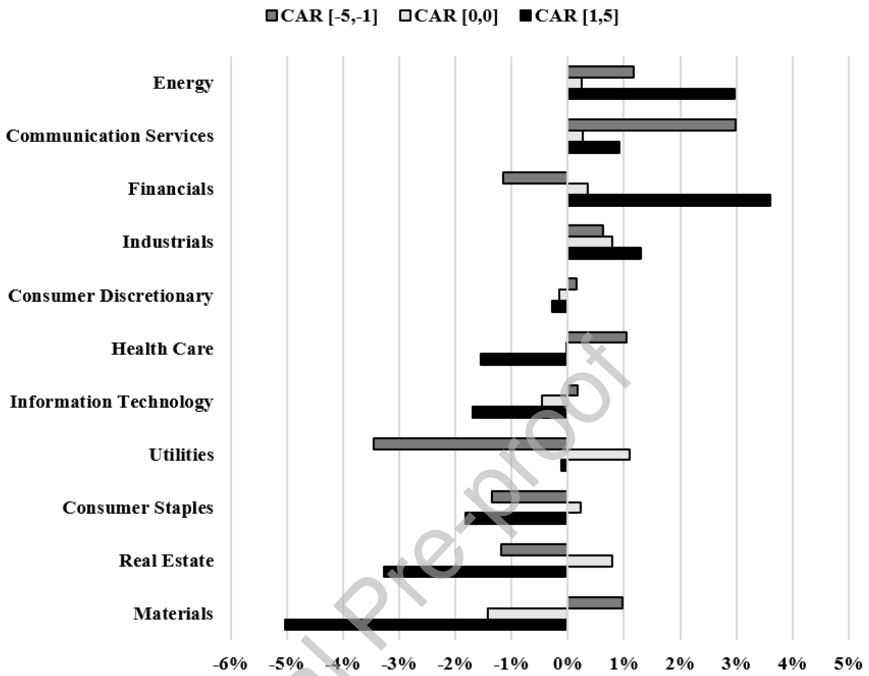
Figure 1. Average CARs for each industry for the event windows [-5,-1], [0,0] and [1,5].
