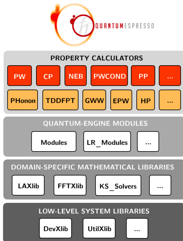
FIG. 1. Schematic illustration of the structure of the QUANTUM ESPRESSO distribution. The non-perturbative codes for SCF, MD, postprocessing and other calculations are those in the first line of the “property calculators” section (highlighted in red), while the linear-response and MBPT codes are in the second line (highlighted in yellow). Low-level layers of the QUANTUM ESPRESSO distribution (as discussed in the text) are also shown.
