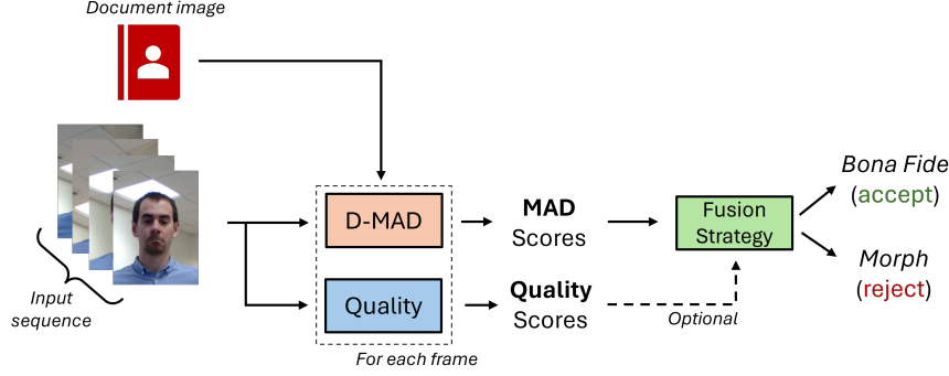
Figure 2: Practical implementation of the V-MAD task. Each frame of the input sequence is analyzed by the same D-MAD model, which receives also the document image as additional input and by a quality tool. Both output MAD and quality scores are then combined through a specific fusion strategy to produce in output the final single score.
