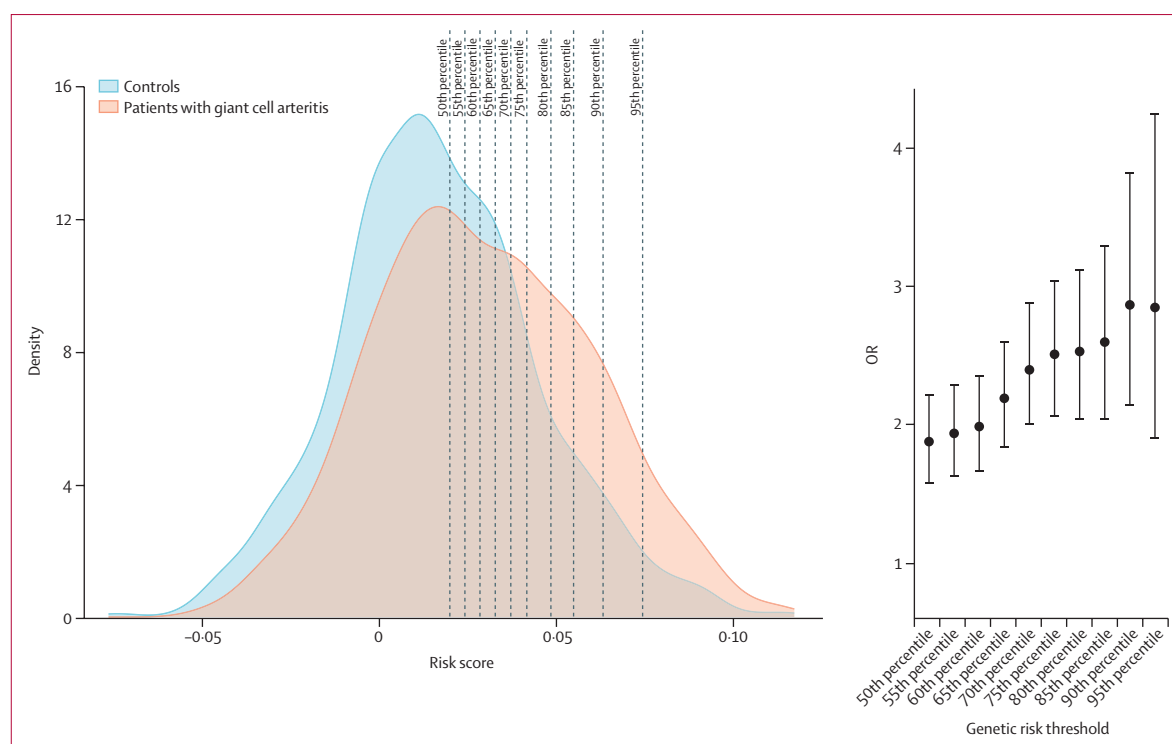
Figure 2: Genetic risk distribution
