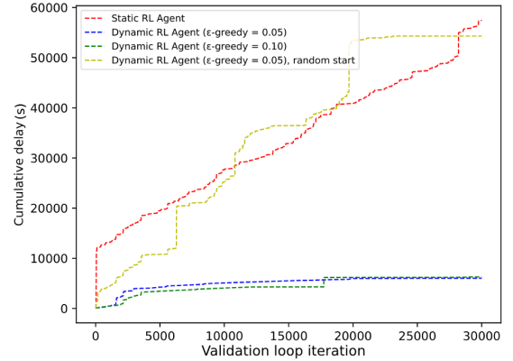
(c) Cumulative delay.
