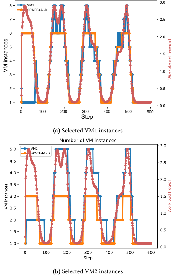
Figure 4. Number of selected VM instances in a 2-components system. Comparison between the choices made by SPACE4AI-D (orange), those by the RL Agent (blue), and the workload (red).
