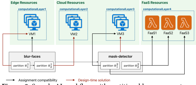
Figure 2. Sample AI workflow with partitionable components and multiple candidate computational layers.
