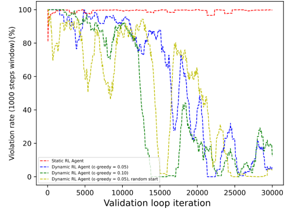
(a) Violation rate.
