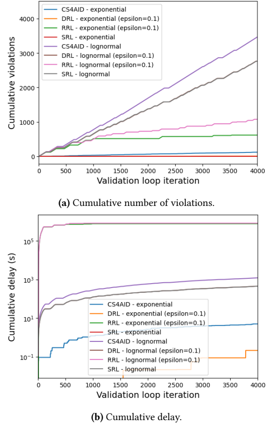
Figure 5. Cumulative number of violations and delay for all Agents, with both exponential and log-normal distributions.
