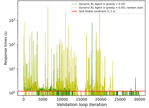
(b) Application response time.
