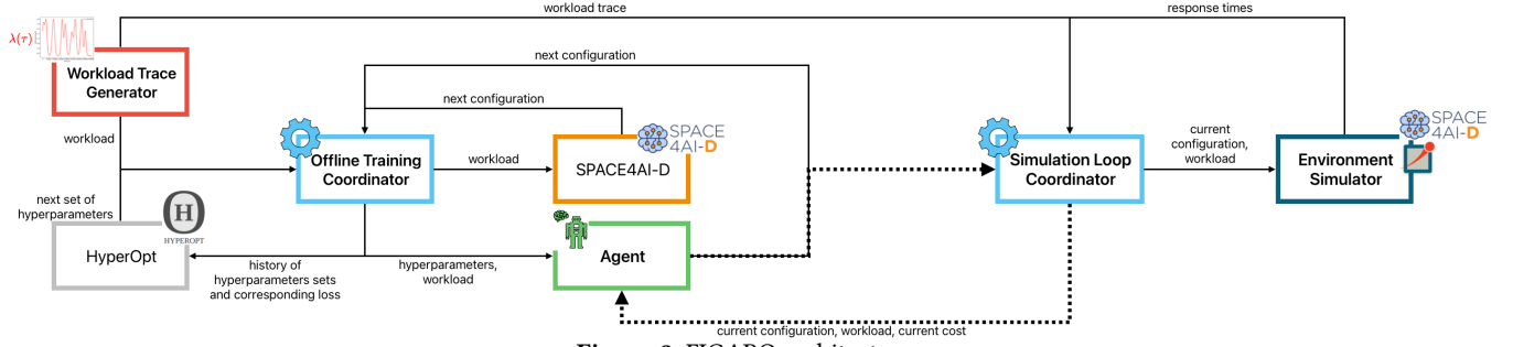
Figure 3. FIGARO architecture.
