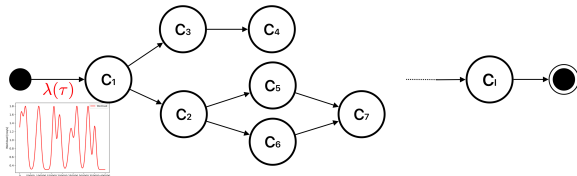
Figure 1. Application DAG.
