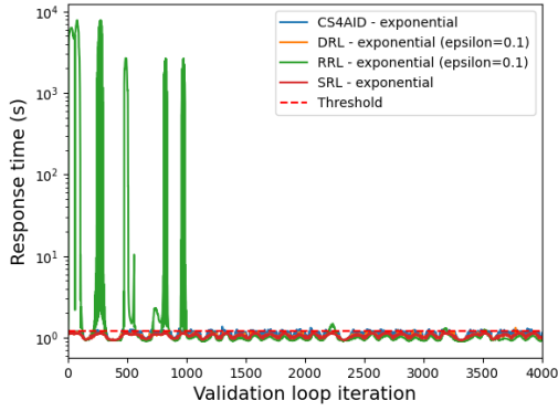
(a) DRL and CS4AID are comparable, while RRL shows very large response times for the first 1000 iterations.
