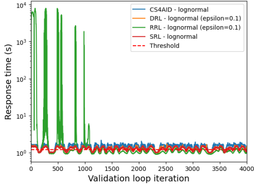
(b) RRL is significantly more inefficient than the others for the first 1000 iterations; for all agents, response times are higher than in the exponential case.
