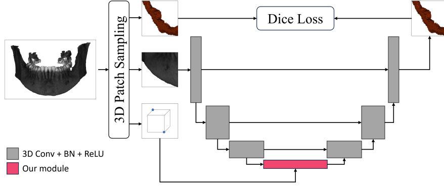
Fig. 3. Proposed Transformer module integrated in the standard 3D U-Net architecture. A detailed visualization of our module is reported in Fig. 4.
