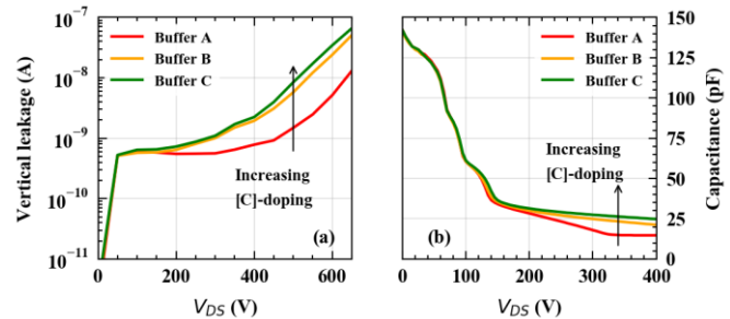
Fig. 4. (a) Vertical leakage current measured at T=25 °C on the DUTs showing different C-doping concentration. The vertical leakage increases while increasing the C-doping level, stemming from a less insulating buffer (i.e., reduced net acceptor concentration). (b) Capacitance-Voltage (C OSS -V) measurement in off-state performed on the three buffer types (A, B and C) with 1 MHz frequency. At relatively high voltage (e.g., 400 V) the output capacitance increases while increasing the C-doping, stemming from a reduced 2-DEG depletion (i.e., reduced negative charge exposed in the Buffer).
