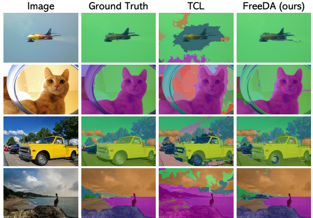
Figure 1. Open-vocabulary segmentation with: (a) TCL [6], which performs end-to-end learning of region-text alignment; (b) our FreeDA , which leverages generated textual-visual embeddings with global-local similarities and does not require any training.
