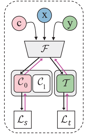
Figure 2. ClusterFix Architecture.
