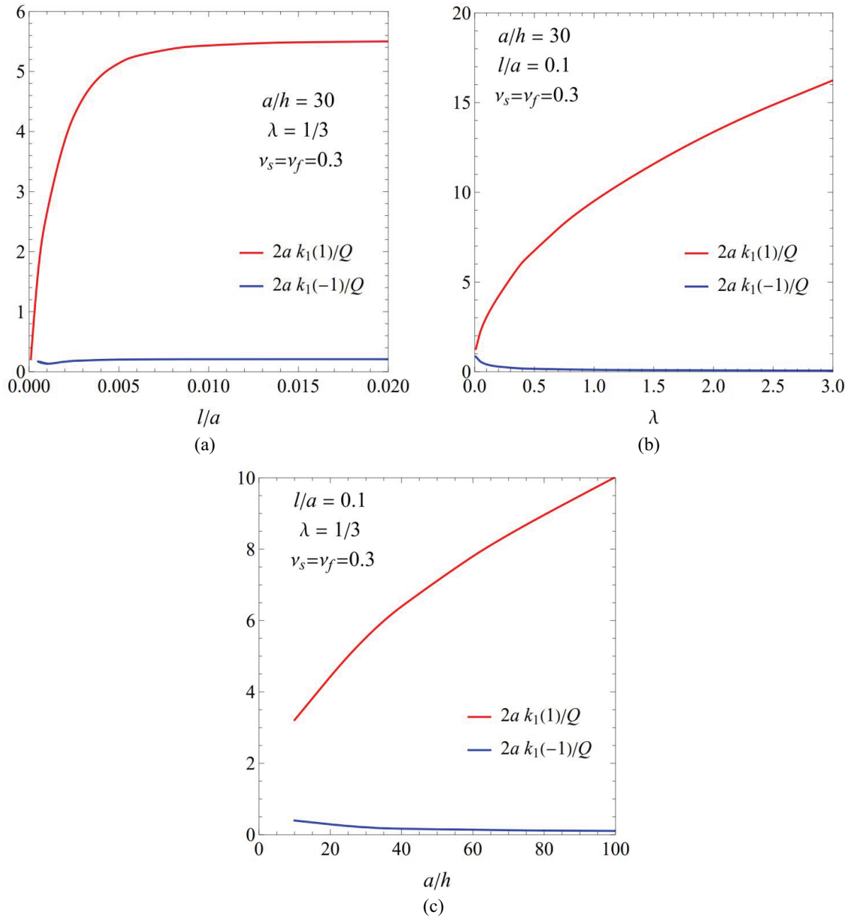
Figure 9. Variations of the strength of stress singularities (a) with the characteristic length ratio l/a , (b) with the stiffness parameter \lambda , and (c) with the geometric ratio a/h , ( \nu_s = \nu_f = 0.3 ).
