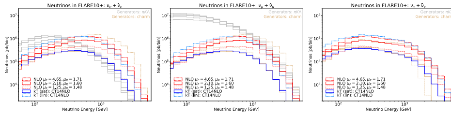
Figure 179. Predictions for the neutrino fluxes going through the 50 cm × 50 cm cross sectional area of the FLArE detector with nominal mass of 10 tonnes. The panels show number of electron (left) muon (center) and tau (right) neutrinos per energy bin passing through the experiments cross section. We show the predictions of different MC event generators as light brown curves. The predictions using the NLO and the k_T factorization approaches are shown in red and blue, respectively. In addition, we show the neutrino fluxes from light meson decays as gray lines.
