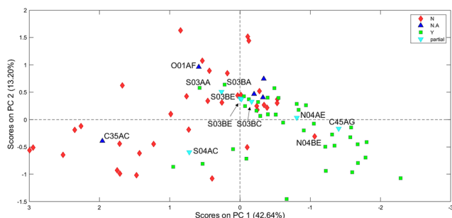
Fig. 3 PC1 vs. PC2 scores plot for the PCA model constructed including all the variables D, A and T for the 83 HS complexes; a symbol legend corresponding to the possibility of undergoing spin transition (Y = yes in green, N = no in red, partial in light blue and N.A. in blue) was applied, and the labels are added only for complexes directly discussed in the text.
