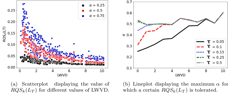
Fig. 7. Plots showing the influence of LWVD and how such parameter can be beneficial for the individual workers to tune internally their parameters.
