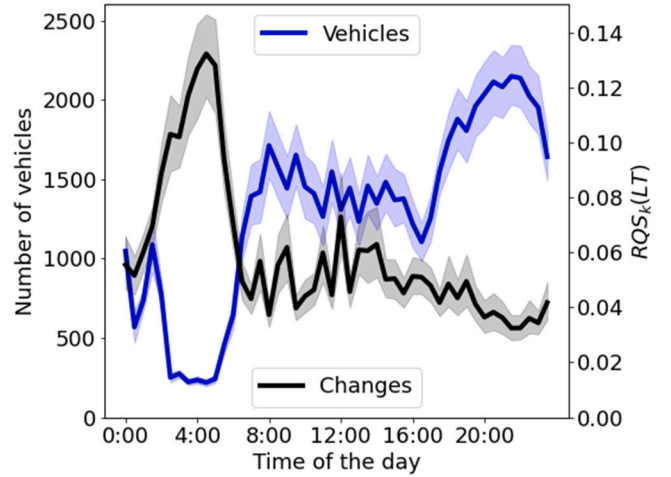
Fig. 5. Number of vehicles and RQS_k(L_T) over time for a simulation covering 24 h.
